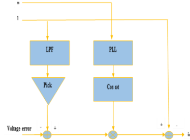
Figure 6: Direct testing and calculating method [37]
