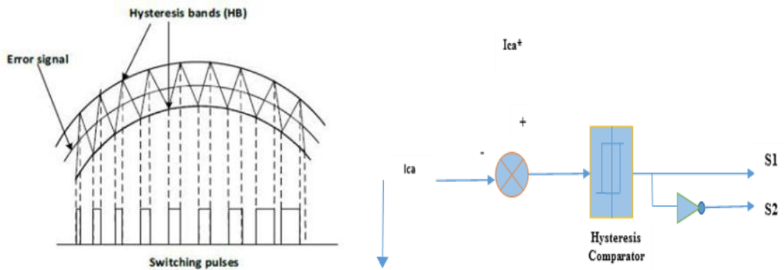
Figure 8: Hysteresis control strategy [15]
