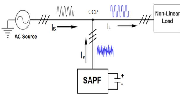
Figure 1: Shunt APF connected to the power system
