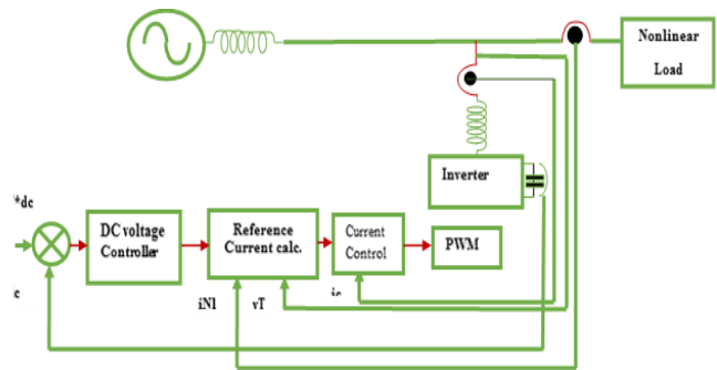
Figure 2: Block diagram of the controller of APF [7]
