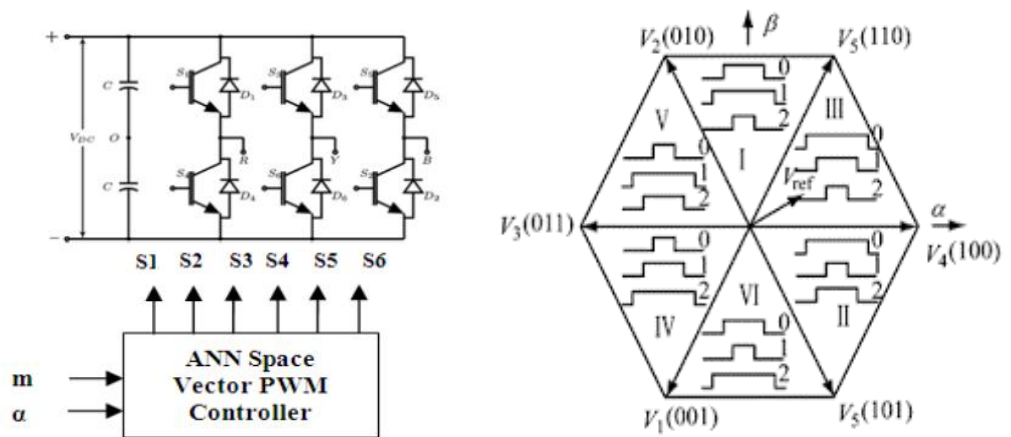
Figure 9: Space vector PWM [36]
