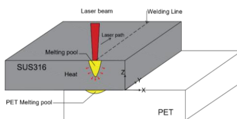
Figure 1: SUS316/PET lap joint diagram
