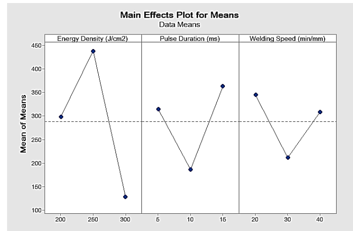
Figure 5: The mean of means plot
