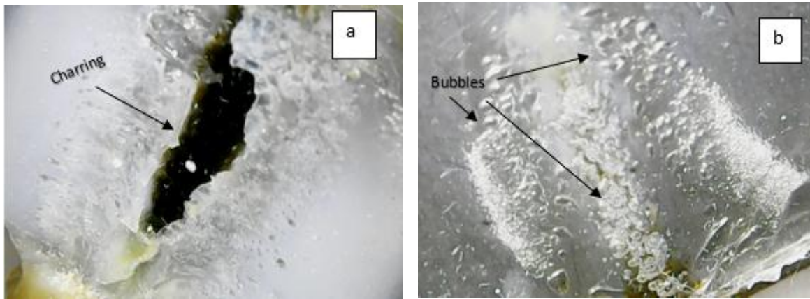
Figure 6: The digital macroscopic morphology of the strongest and weakest joint
