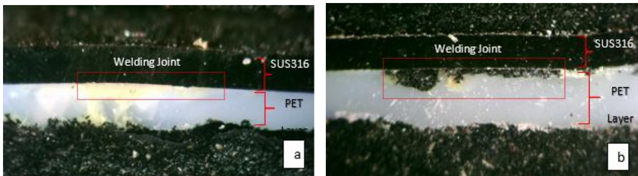
Figure 8: The microscope pictures of the strongest and weakest joints
