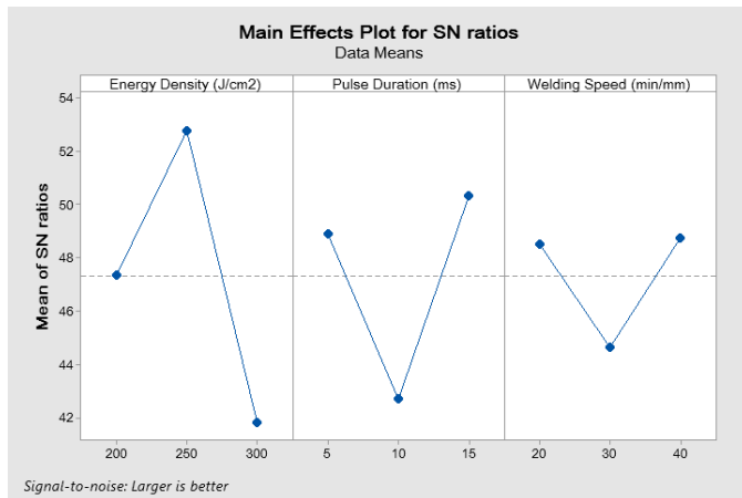
Figure 4: The S/N ratio of the joint force
