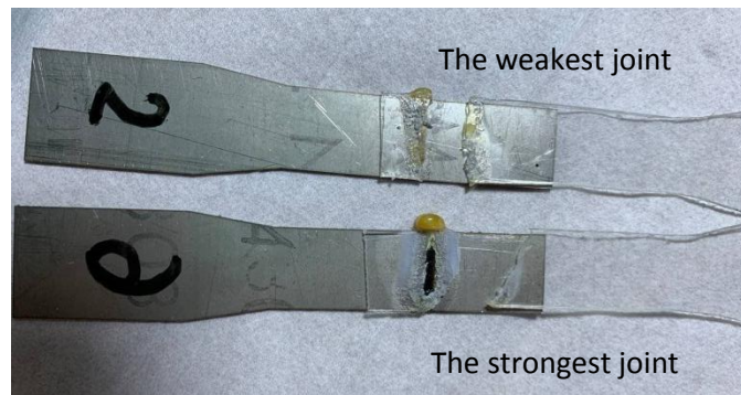
Figure 7: The strongest and weakest joints after the tensile shear test
