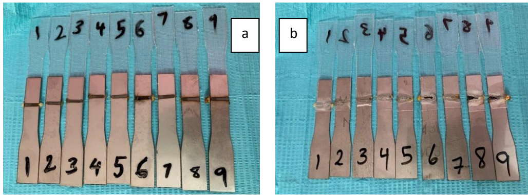
Figure 2: A lap joint of SUS316 and PET
