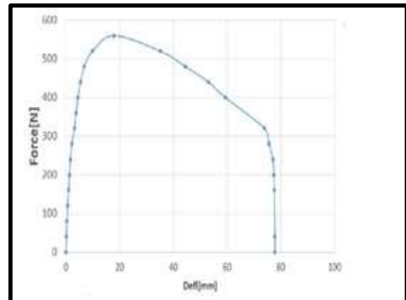
Figure 21: Force-deflection diagram
