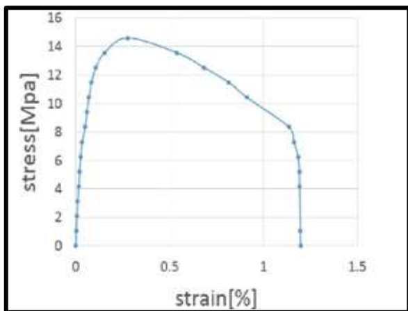
Figure 22: Stress-strain diagram
