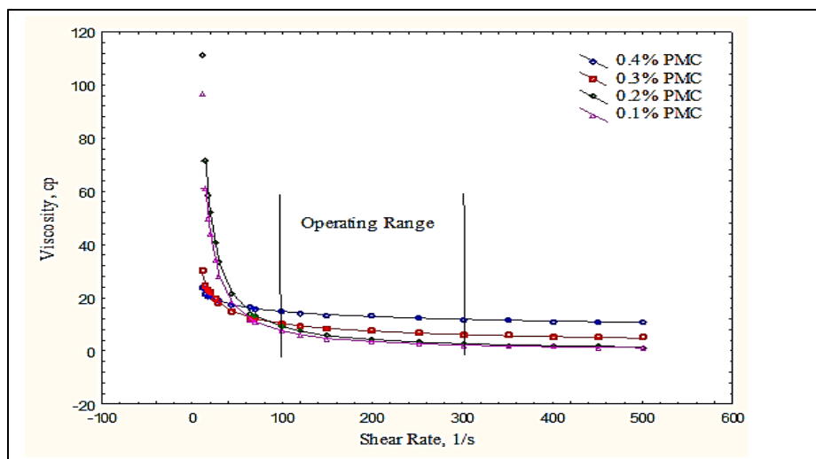
Figure 1: Effective shear rates (1/s) with Viscosity (cp)
