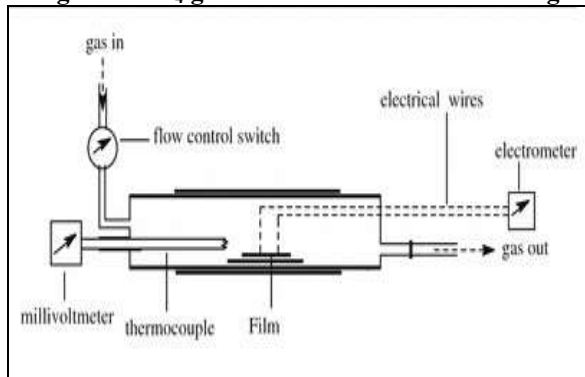
Figure 3: Electric Circuit of gas sensor.
