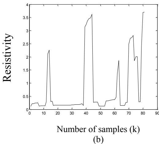
Figure4. Input-output data resulted from the real-time experiment (a) input signal (concentration of the pollutant gas (CH 4 )) and (b) output response (resistivity of the gas detector NiO nano film).
