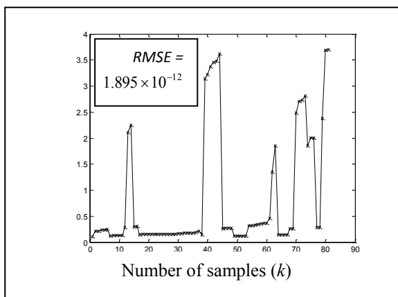
Figure 7: Real response (solid line) and the developed model response (×-marks).
