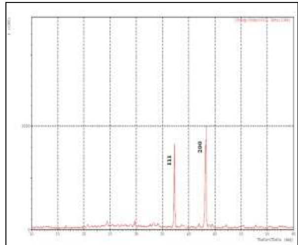
Figure 5: XRD diffractogram of NiO nano film.
