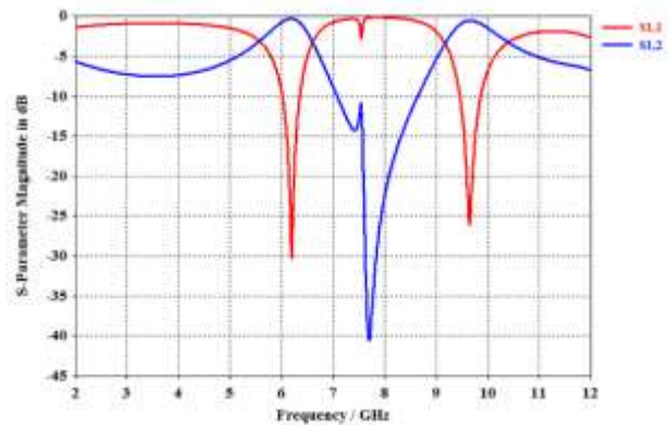
Figure 8: The simulated S11 and S12 responses of the folded open loop B-shaped slot BPF.
