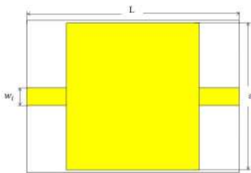
Figure 1: CST MWS model for the proposed BPF (top layer)
