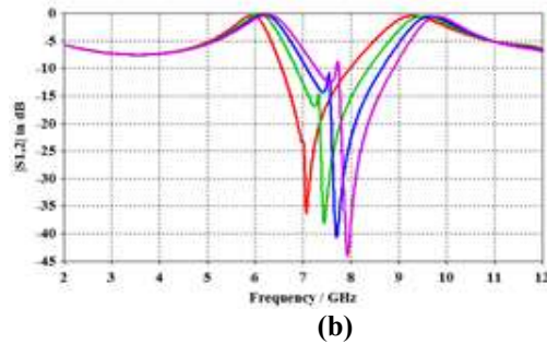
Figure 6: Parametric study of the proposed filter with g as a parameter: (a) Input reflection coefficient (S11), and (b) Insertion loss (S12).
