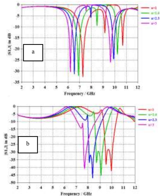
Figure 4: Parametric study of the proposed filter with v as a parameter : (a) Input reflection coefficient(S11), and (b) Insertion loss (S12)
