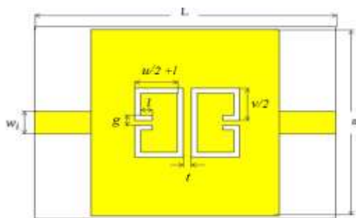
Figure 3: The layout of the folded open loop B-shaped slot BPF
