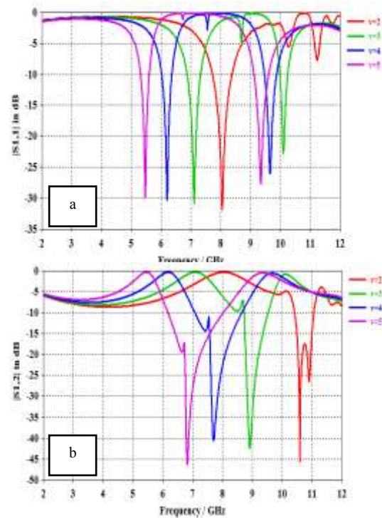
Figure 4: Parametric study of the proposed filter with v as a parameter : (a) Input reflection coefficient(S11), and (b) Insertion loss (S12)
