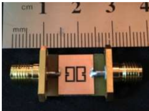
Figure 9: Photograph of the fabricated prototype of the folded open loop B-shaped slot BPF.
