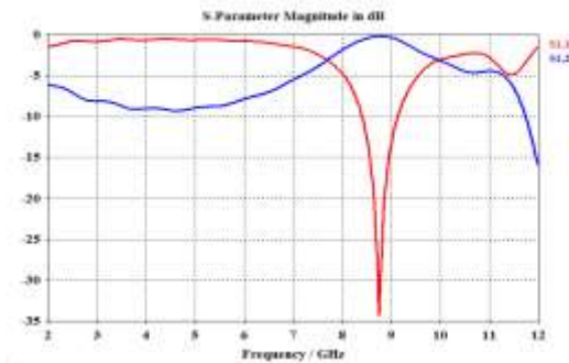
Figure 2: Simulated S11 and S12 results of the BPF
