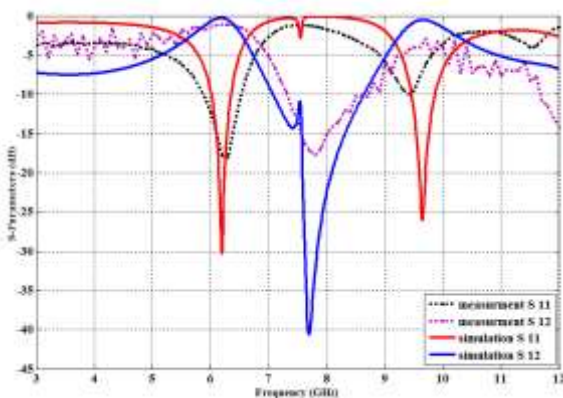
Figure 10: Comparison between the simulated and the measured S-parameters for the fabricated folded open loop B-shaped slot BPF.
