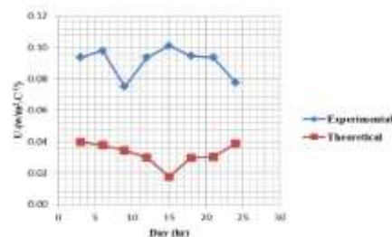
Figure 13: Variation of actual and theoretical of heat transfer coefficient with time for AR=15
