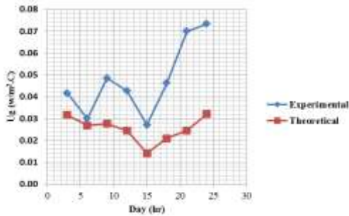
Figure 15: Variation of actual and theoretical of heat transfer coefficient with time for AR=10 argon
