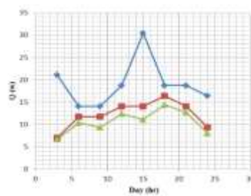
Figure 10: Change of heat transfer rate with time
