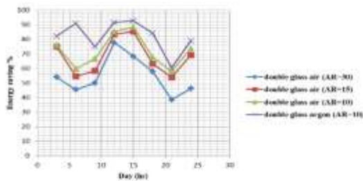
Figure 16: Energy saving of the heat transfer with time
