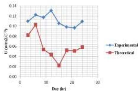
Figure 13: Variation of actual and theoretical of heat transfer coefficient with time for AR=15
