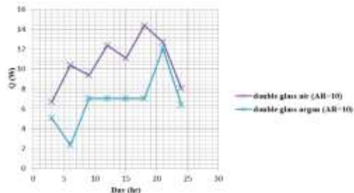
Figure 11: Change of heat transfer rate with time at constant AR
