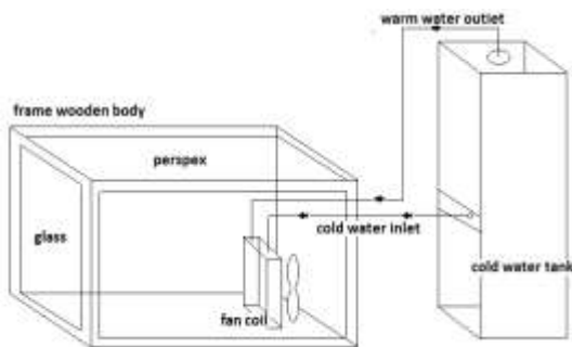
Figure 2: Schematic diagram of the experimental rig
