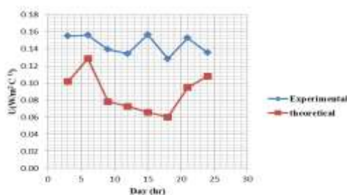
Figure 12: Variation of actual and theoretical of heat transfer coefficient with time for AR=30
