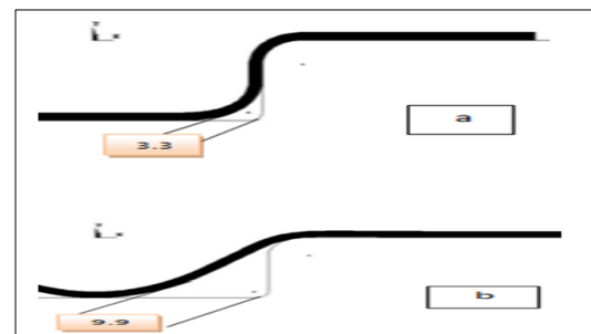
Figure 10: Shape conformation of the final tube at corner radius (a) with axial feeding, (b) without axial feeding.
