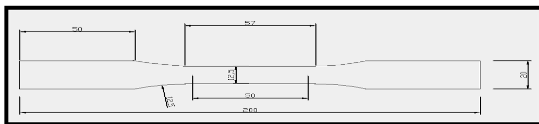
Figure 2: The dimensions of the tensile test specimen according to ASTM standard E8M specification.
