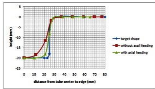
Figure 8: Shape conformation of the final tube from center to the edge after forming process.
