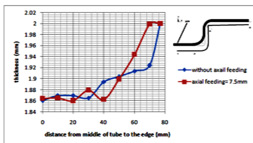
Figure 7: The variations in thickness on the tube wall from middle tube to the edge, for two cases (without axial feeding and with axial feeding value (7.5mm)).
