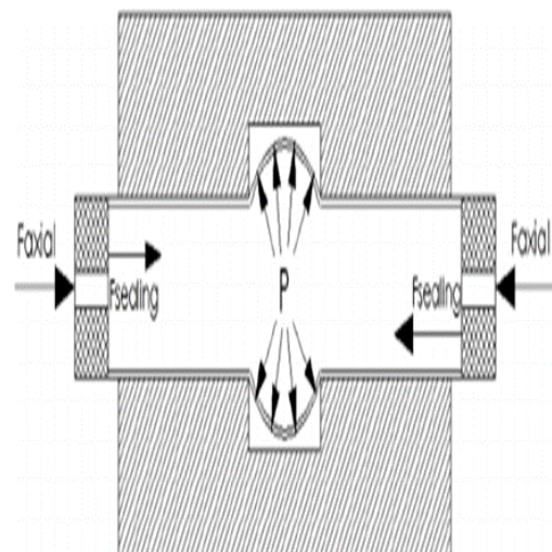
Figure 1 Tube hydroforming process
