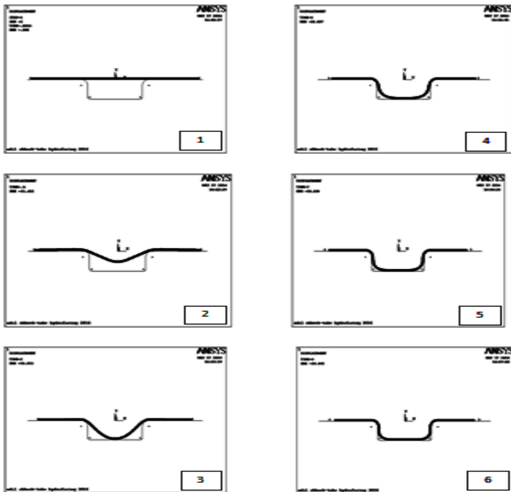
Figure 4: Different stages of material deformation during simulation in tube hydroforming process.
