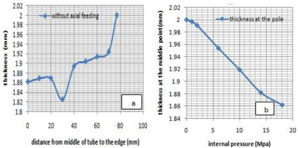
Figure 6: The thickness distribution on the tube wall. 6a, thickness distribution from middle to the edge tube. 6b, variation in the pole thickness during the hydroforming process.
