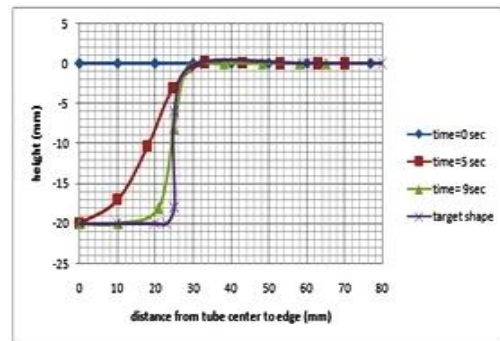
Figure 9: Shape conformation of the tube from center to the edge throughout the forming process.
