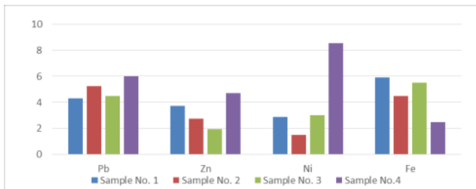
Figure 6: The measured values of Pb, Zn, Ni, and Fe samples
