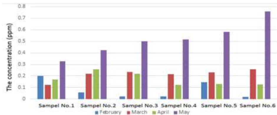
Figure 10: SO 2 values of the four month
