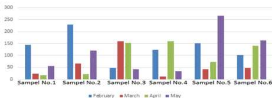
Figure 14: Represent the difference value for PM_{2.5} in four month
