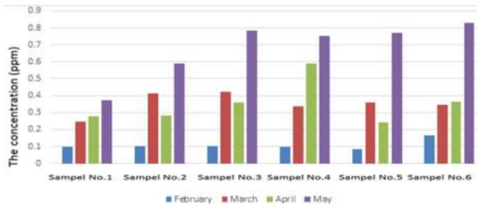
Figure 11: NO 2 values of the four month
