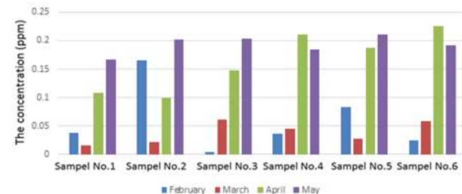
Figure 12: VOC s values of the four month
