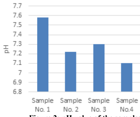
Figure 2: pH value of the samples
