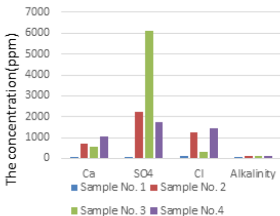
Figure 4: The obtained values of Ca 2+ , SO 4 2- , and Cl samples
