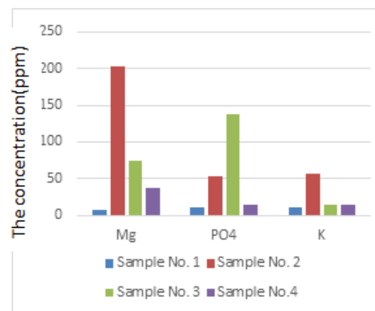
Figure 5: The obtained values of Mg 2+ , PO 4 3- , and K + samples
