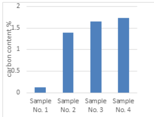
Figure 3: carbon content value of the samples
