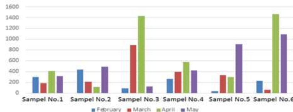
Figure 15: PM_{10} values of the four month
