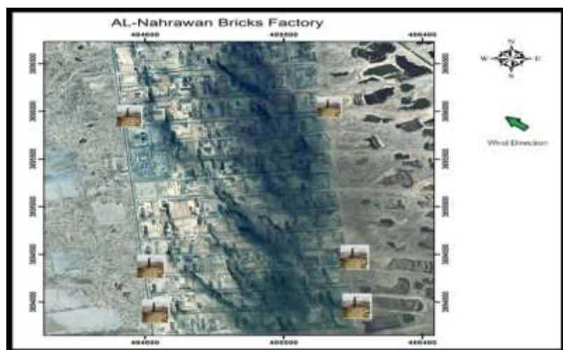
Figure 1: Spot 7 Satellite image (with resolution 1.5m) in 6/10/2014 of AL-Nahrawan show the Location Samples
