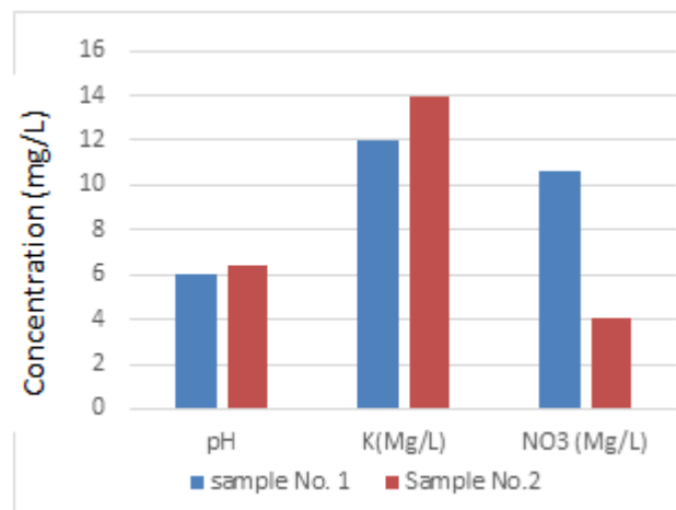
Figure 8: The measured values of pH, K + , and NO 3 - samples
