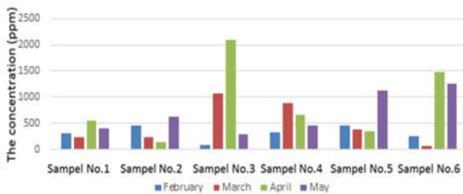
Figure 13: TSP values of the four month
