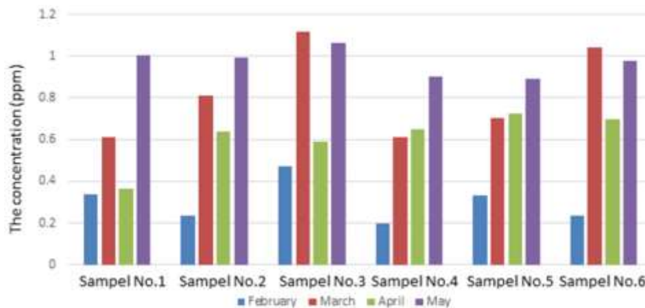
Figure 9: H 2 S values of the four month
