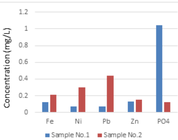
Figure 7: The measured values of Fe 3+ , Ni 2+ , Pb 2+ , Zn 2+ , and PO 4 3- samples
