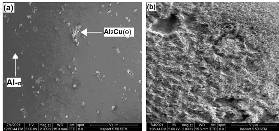
Figure 3: The SEM image of the annealed sample: (a) Before the erosion test, (b) After the erosion test
