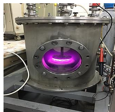
Figure 2: Plasma nitriding device
