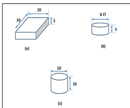
Figure 1: Dimensions of samples for (a) erosive wear and hardness test, (b) scanning electron microscope (SEM), and (c) X-ray diffraction (XRD), optical microscope: All dimensions in mm
