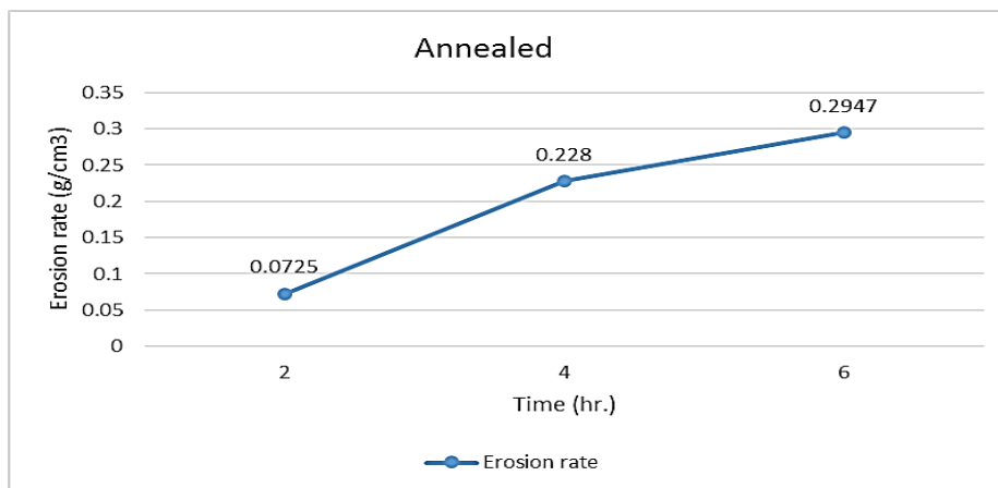
Figure 6: The erosion wear rate of annealed samples at 45° impact angle
