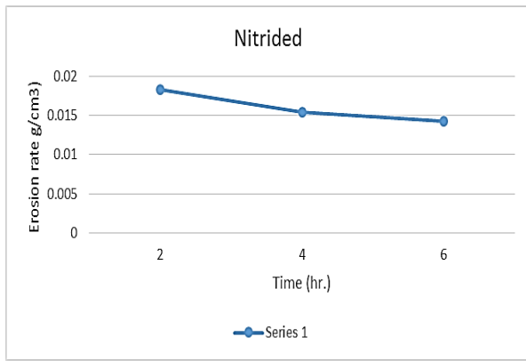
Figure 7: The erosion wear rate of nitrided samples
