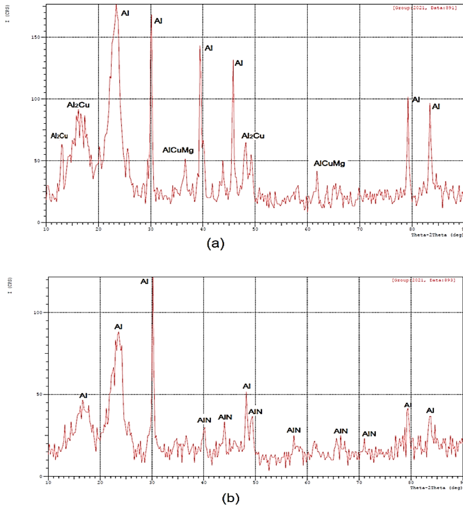
Figure 5: XRD Patterns: (a) Al-Cu 2024 after annealing, (b) After plasma nitriding
