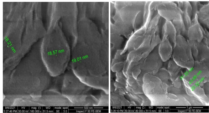
Figure 2: Field Emission Scan Electronic Microscope (FESEM) photo for Nano clay.
