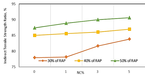
Figure 8: Influence of Nano-clay percent on Indirect Tensile Strength Ratio.
