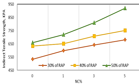
Figure 7: Influence of the amount of Nanoclay on the Indirect Tensile Strength for the Conditioned Sample.
