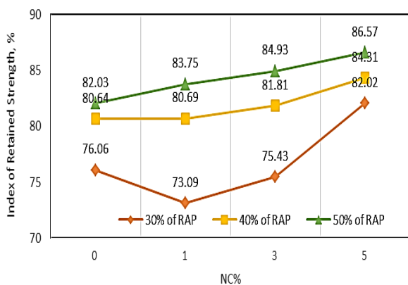
Figure 5: The Impact of Nono-clay Content on the Index of Retained Strength
