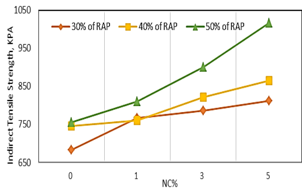
Figure 6: Influence of Nono-clay percent on the Indirect Tensile Strength for theUnconditioned Sample.
