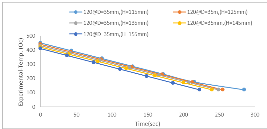
Figure 7: Temperature-time Cooling Profile @ 120°C for D=35mm and H=115, 125, 135, 145 and 155mm
