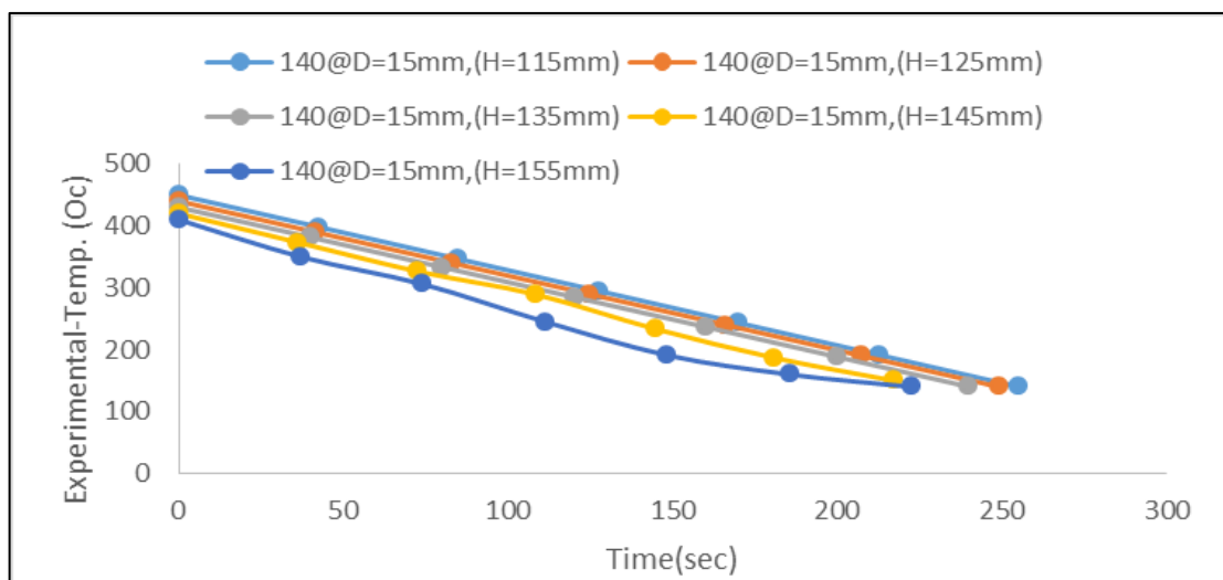
Figure 5: Temperature-time Cooling Profile @ 140°C for D=15mm and H=115, 125, 135, 145 and 155mm
