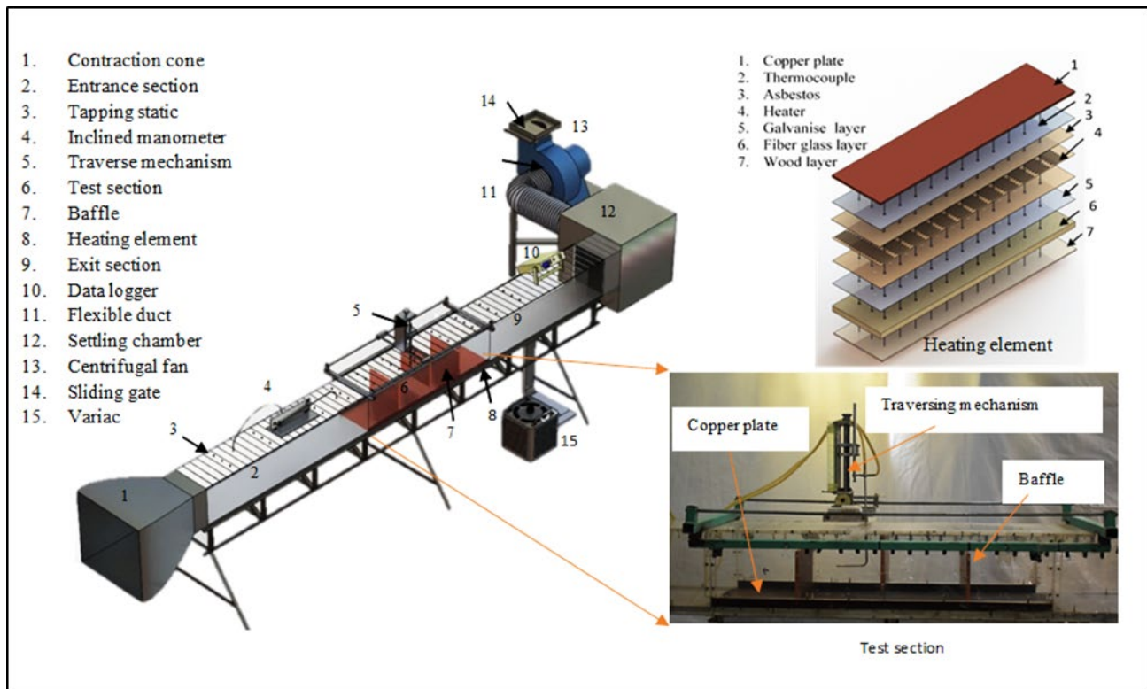
Figure 1: Experimental setup
