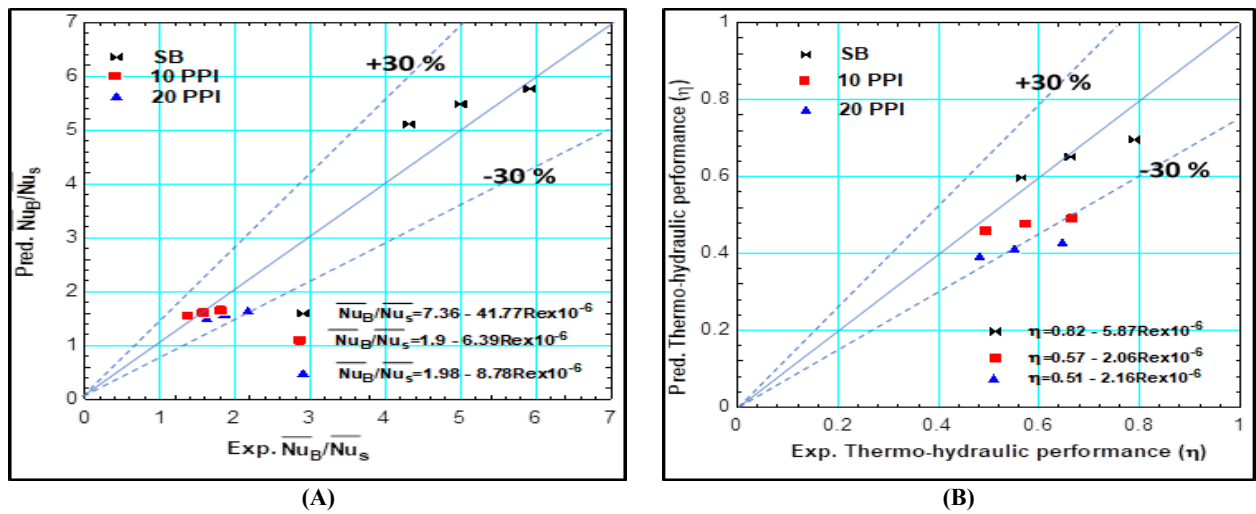
Figure 12: Comparison of the present experimental data with a correlation of [11]: (A) \frac{\overline{Nu}_B}{\overline{Nu}_s} and (B) Thermo-hydraulic performance
