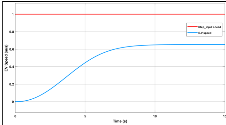
Figure 2: The response EV model without controller
