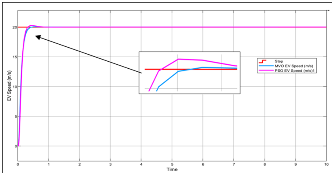
Figure 6: Speed control response with PID controllers and PSO and MVO optimization
