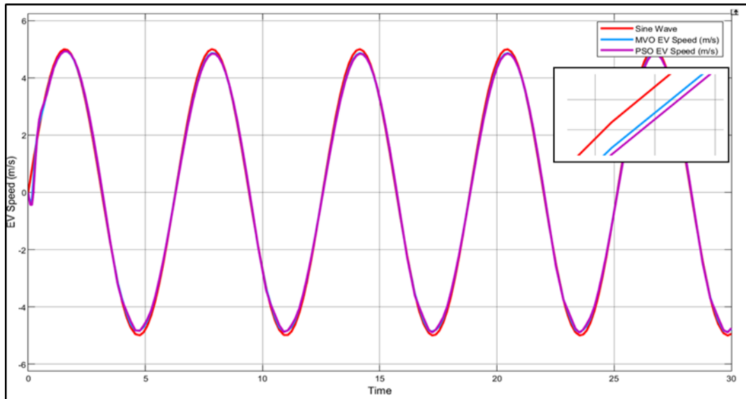
Figure 7: Speed control response with PID controllers and PSO and MVO optimization
