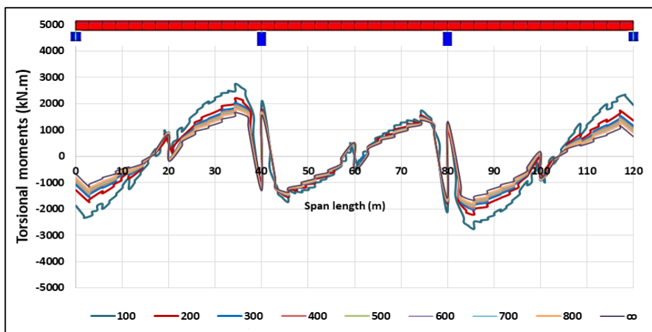
Figure 6: Outer face torsional moments along the span under central loading
