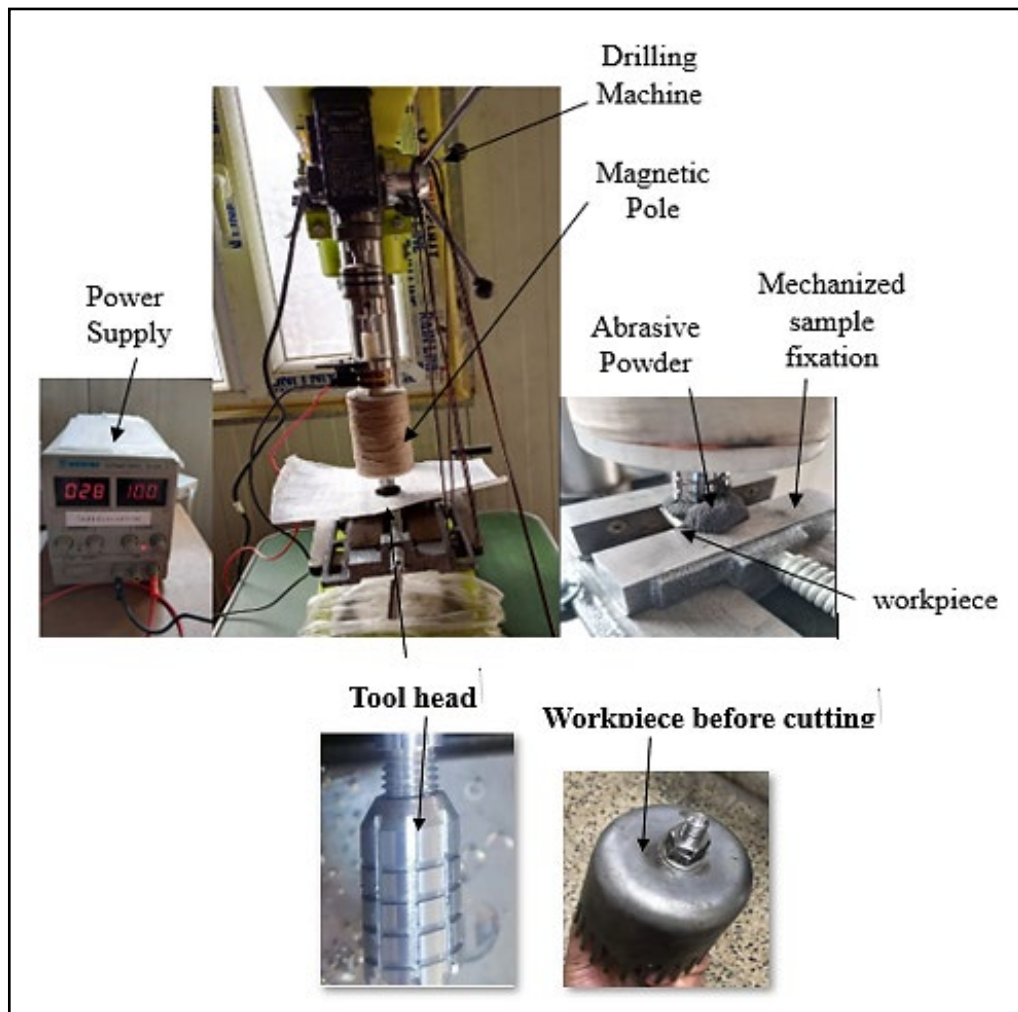
Figure 2: Experimental Setup
