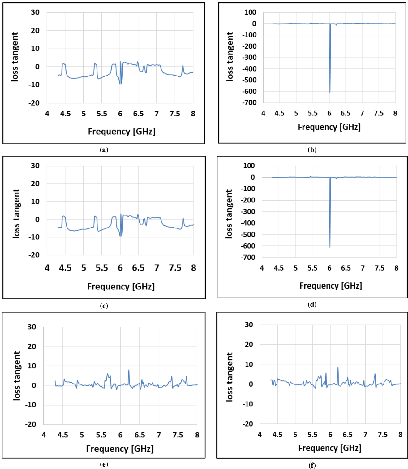
Figure 5: The tangent loss calculated in the C-band frequency for (a) 10% volume fraction Zn_{1-x}Cu_xWO_4(x=0) /epoxy composite (b) 10% volume fraction Zn_{1-x}Cu_xWO_4(x=0.03) /epoxy composite (c) 10% volume fraction Zn_{1-x}Cu_xWO_4(x=0) /polyurethane composite (d) 10% volume fraction Zn_{1-x}Cu_xWO_4(x=0.03) /polyurethane composite (e) 10% volume fraction Zn_{1-x}Cu_xWO_4(x=0) /silicone rubber composite (f) 10% volume fraction Zn_{1-x}Cu_xWO_4(x=0.03) /silicone rubber composite
