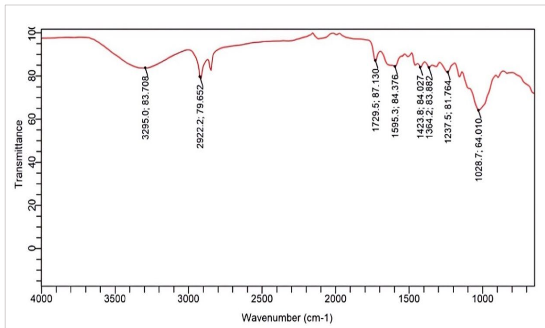
Figure 2: FTIR Spectral of Raffia Palm Fibres
