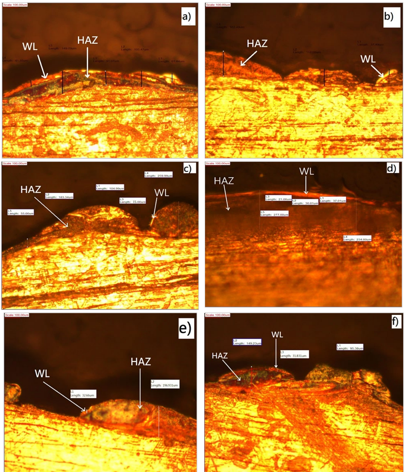
Figure 6: Microscopically pictures for measured WLT and HAZ a) I 16 A, Ton 200 μs, Con. 0 g/l, MF 0.2 T. b) I 8 A, Ton 200 μs, Con. 0 g/l, MF 0.2 T. c) I 16 A, Ton 200 μs, Con. 2 g/l, MF 0.2 T. d) I 8 A, Ton 200 μs, Con. 2 g/l, MF 0.2 T. e) I 16 A, Ton 200 μs, Con. 4 g/l, MF 0.2 T. f) I 8 A, Ton 200 μs, Con. 4 g/l, MF 0.2 T
