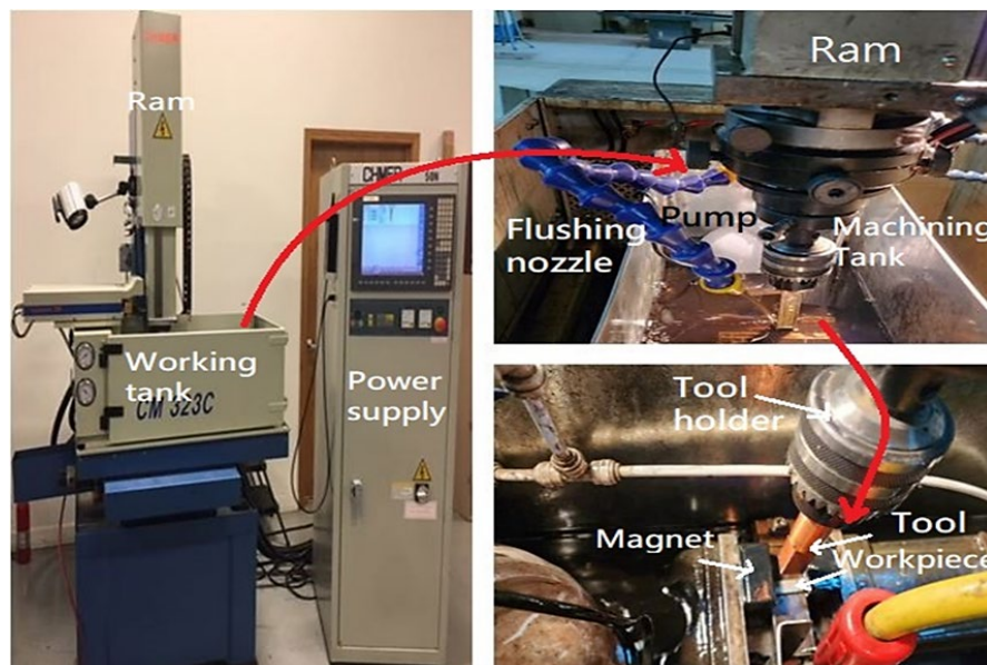
Figure 3: Experimental setup
