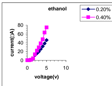
Figure (4). current-voltage curves for ethanol
