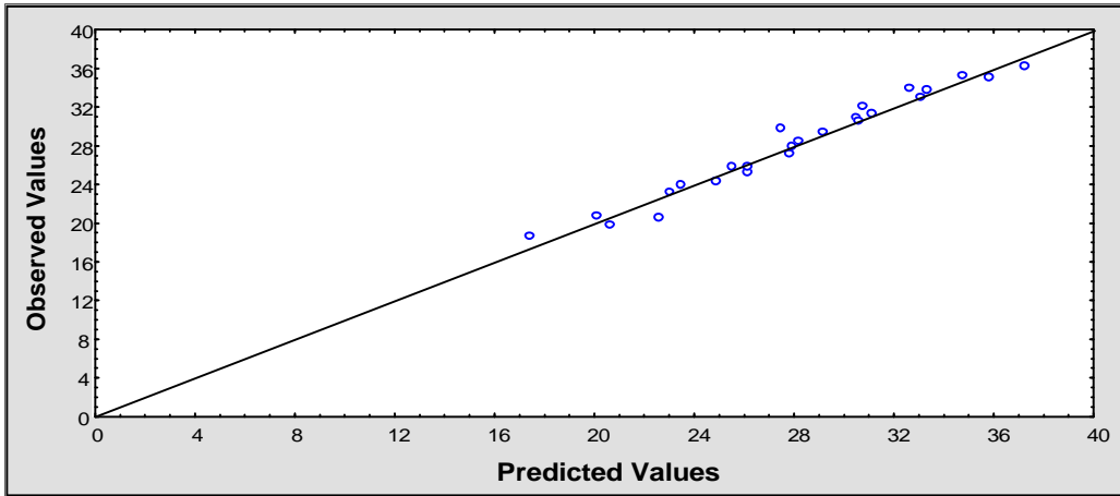
Figure (13) Experimental versus predicted values for Eq.(1)
