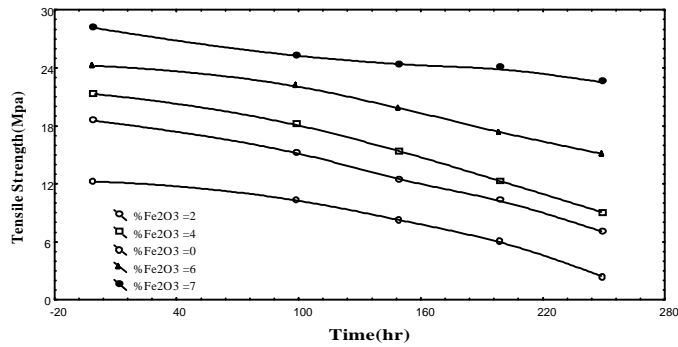
Figure1 Tensile strength of LDPE as function of exposure times at different wt% of Fe 2 O 3 and constant TiO 2 content.(7% wt).
