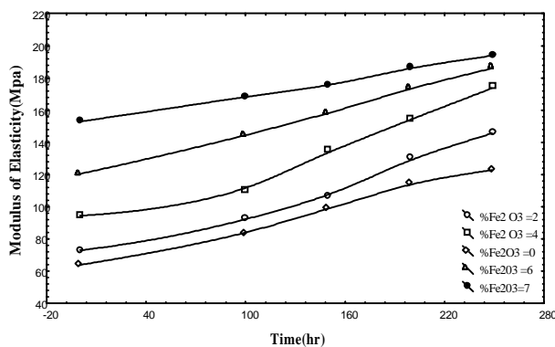
Figure. 11 %Modulus of elasticity of LDPE as a function of exposure times at different wt.% Fe_2O_3 , TiO_2 and constant TiO_2 content
