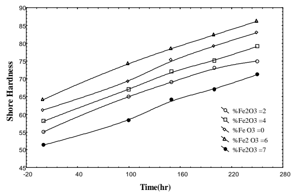
Figure. 10 Shore Hardness of LDPE as a function of exposure times at different wt.% Fe_2O_3 and constant TiO_2 content
