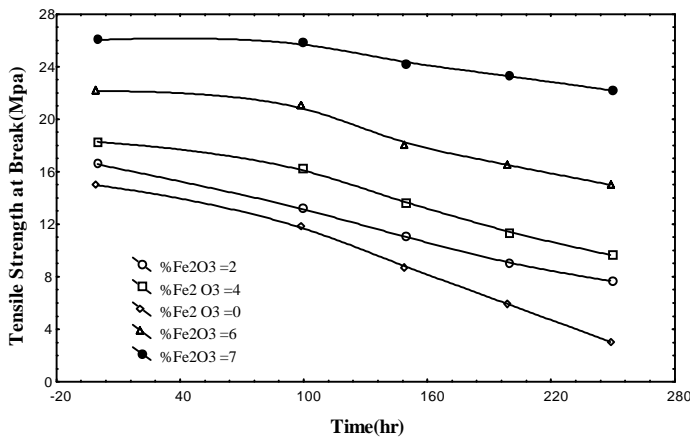
Figure 3 Tensile strength at break of LDPE as a function of exposure times at different wt.% of Fe 2 O 3 and constant TiO 2 content (7% wt).
