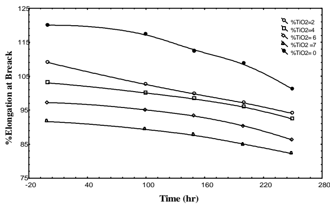
Figure 5 %Elongation of LDPE as a function of exposure times at different wt.% TiO 2 and constant Fe 2 O 3 content
