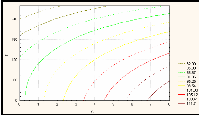
Figure (15) Contour plot obtained from (Exposure times,wt% of Fe 2 O 3 , modulus of elasticity).
