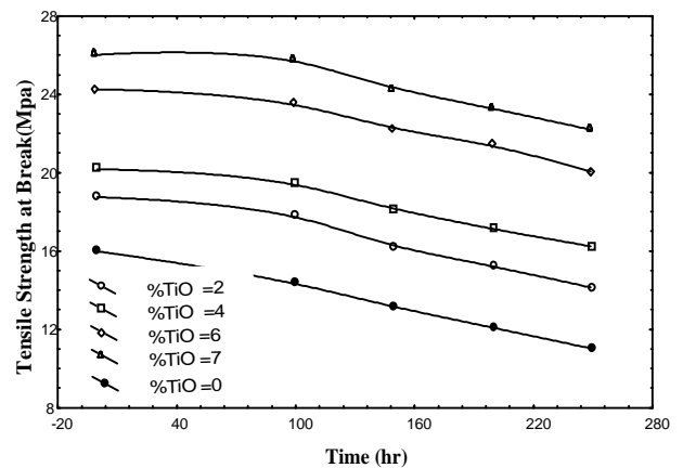
Figure 4 Tensile strength at break of LDPE as a function of exposure times at different wt.% of TiO 2 and constant Fe 2 O 3 content (7% wt) .
