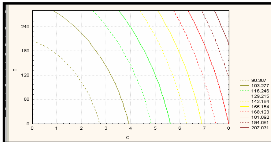
Figure (16) Contour plot obtained from (Exposure times,wt% of TiO 2 , modulus of elasticity)
