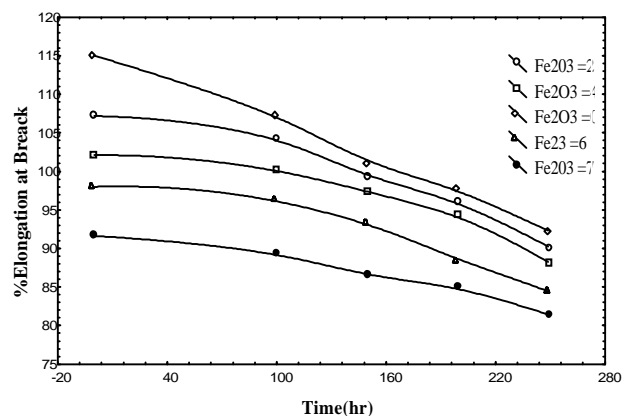
Figure 6 %Elongation of LDPE as a function of exposure times at different wt.% Fe 2 O 3 and constant TiO 2 content (7% wt).
