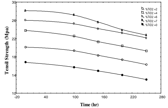
Figure 2 Tensile strength of LDPE as function of exposure times at different wt.% of TiO 2 and constant Fe 2 O 3 content.(7% wt).
