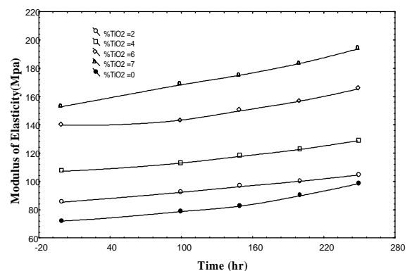
Figure 12 %Modulus of elasticity of LDPE as a function of exposure times at different wt.% TiO_2 and constant Fe_2O_3 content
