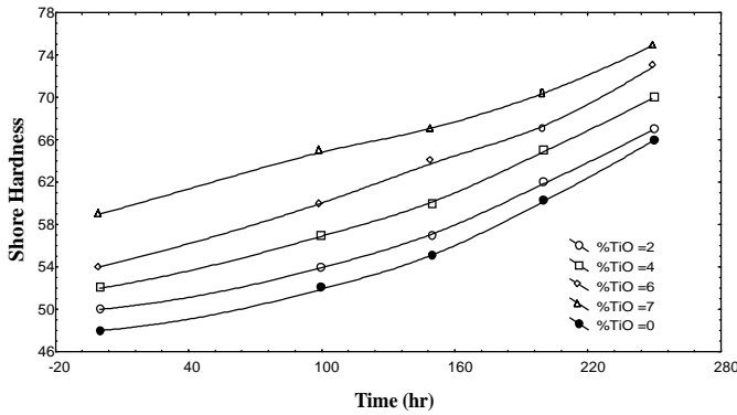
Figure 9 Shore Hardness of LDPE as a function of exposure times at different wt.% TiO_2 and constant Fe_2O_3 content
