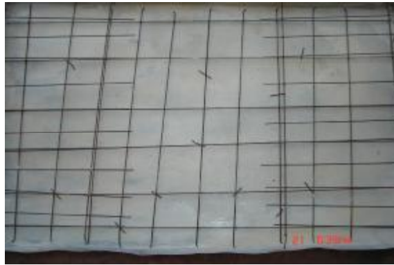
Photo (3) Details of the reinforcement mesh of slab S_3 (case3).
