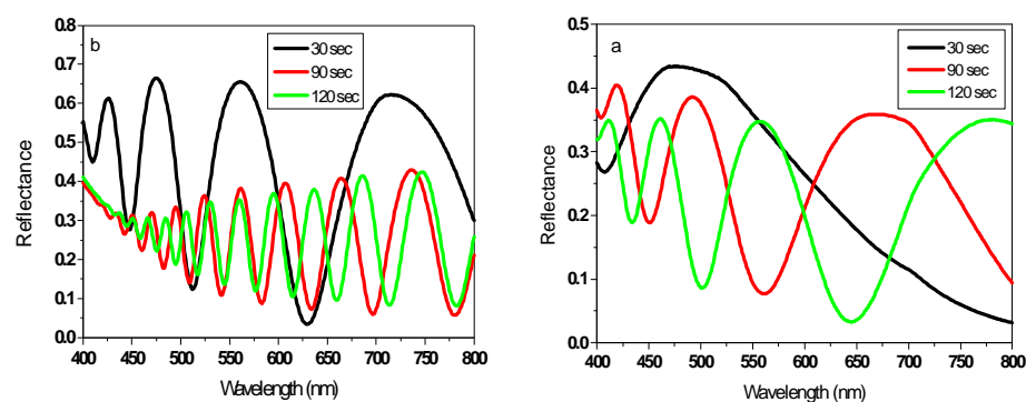
Figure (1) Experimental and reflectance vs. wavelength for different time etching and different current density a) 5mA/cm 2 b) 45mA/cm 2
