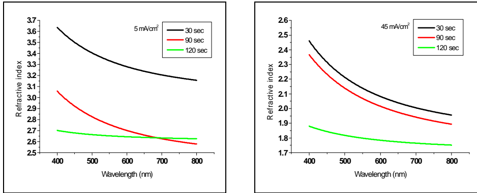
Figure (2) Refractive index of a porous silicon layer simulated with a thin film Cauchy model for different Current densities. a) 5mA/cm 2 b) 45mA/cm 2
