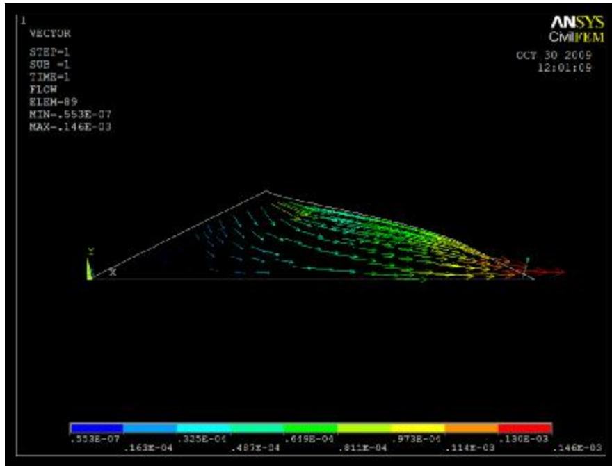
Figure (5) Flow pattern through dam body – CivilFEM output
