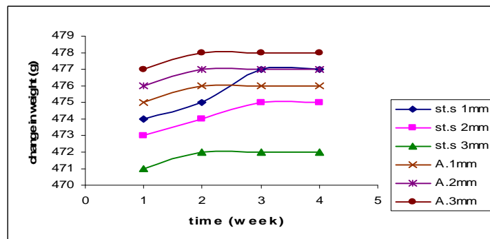
Figure (11) The effect of primer thickness of the chemical activity of epoxy/alumina primer under H_2SO_4 solution field at 28 days and 50^\circ C .
