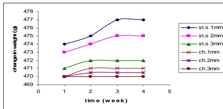
Figure (12) The effect of epoxy/charcoal thickness on chemical activity primer under H_2SO_4 solution field at 28 days and 50^\circ C .
