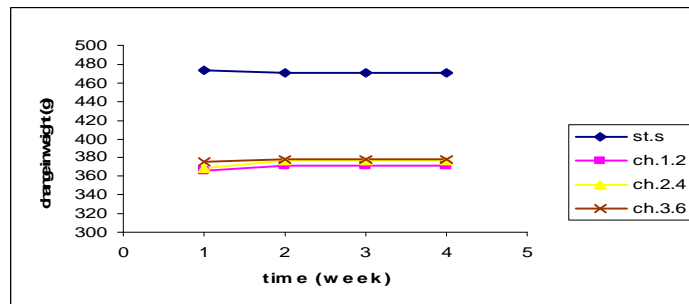
Figure (10) The effect of type and concentration of primer charcoal additive on chemical activity of primer under H_2SO_4 solution field at 28 days and 50^\circ C .
