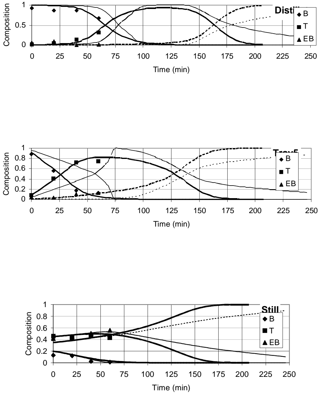
Figure (9): Experimental and Simulation Results of Equilibrium and Nonequilibrium Models Experiment no-4 Table (3). (Points \equiv Exp., Soft lines \equiv EQ model, and Bold Lines \equiv NEQ model)
