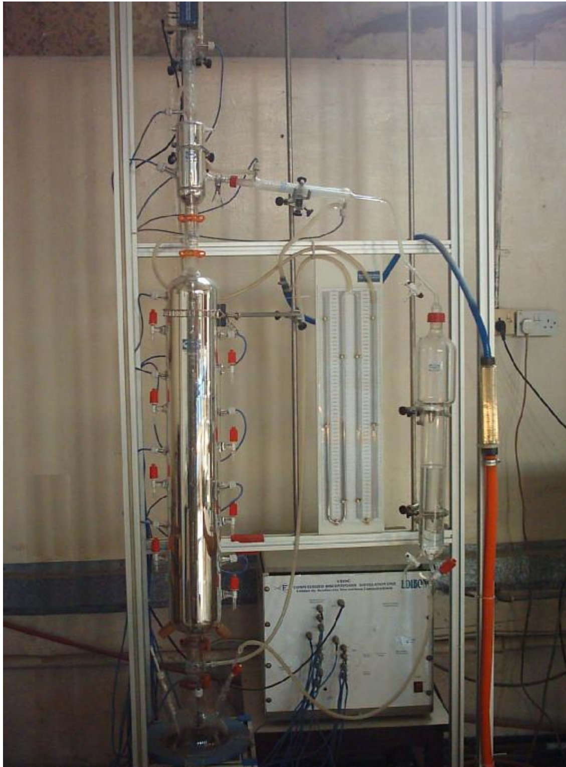
Figure (5): Photograph for The Experimental Rig of Batch Distillation Column
