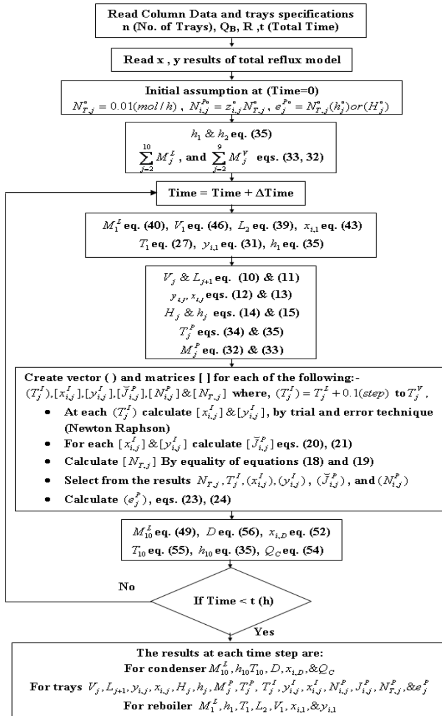
Figure (4): The Flow Chart of Solution Steps of Non-equilibrium Stage Model
