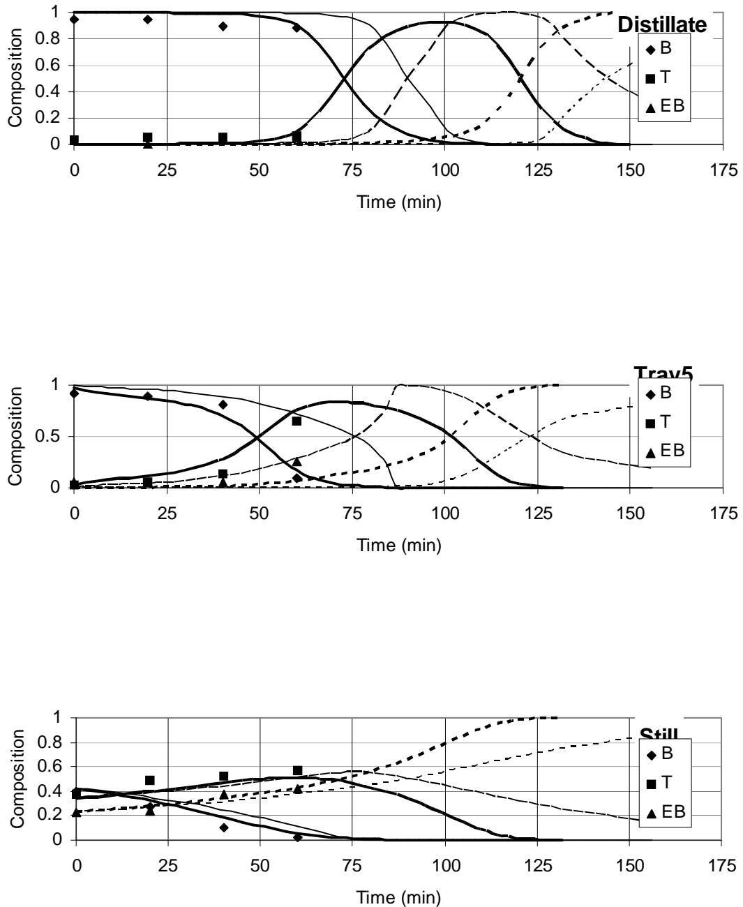
Figure (11): Experimental and Simulation Results of Equilibrium and Nonequilibrium Models Experiment no-6 Table (3). (Points \equiv Exp., Soft lines \equiv EQ model, and Bold Lines \equiv NEQ model)
