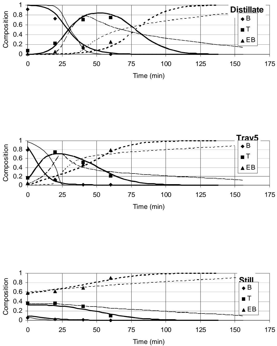
Figure (10): Experimental and Simulation Results of Equilibrium and Nonequilibrium Models Experiment no-5 Table (3). (Points \equiv Exp., Soft lines \equiv EQ model, and Bold Lines \equiv NEQ model)
