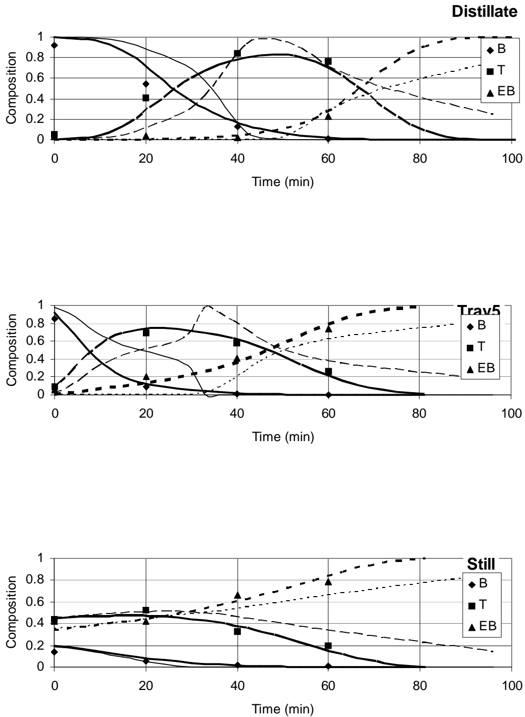
Figure (7): Experimental and Simulation Results of Equilibrium and Nonequilibrium Models Experiment no-2 Table (3). (Points \equiv Exp., Soft lines \equiv EQ model, and Bold Lines \equiv NEQ model)
