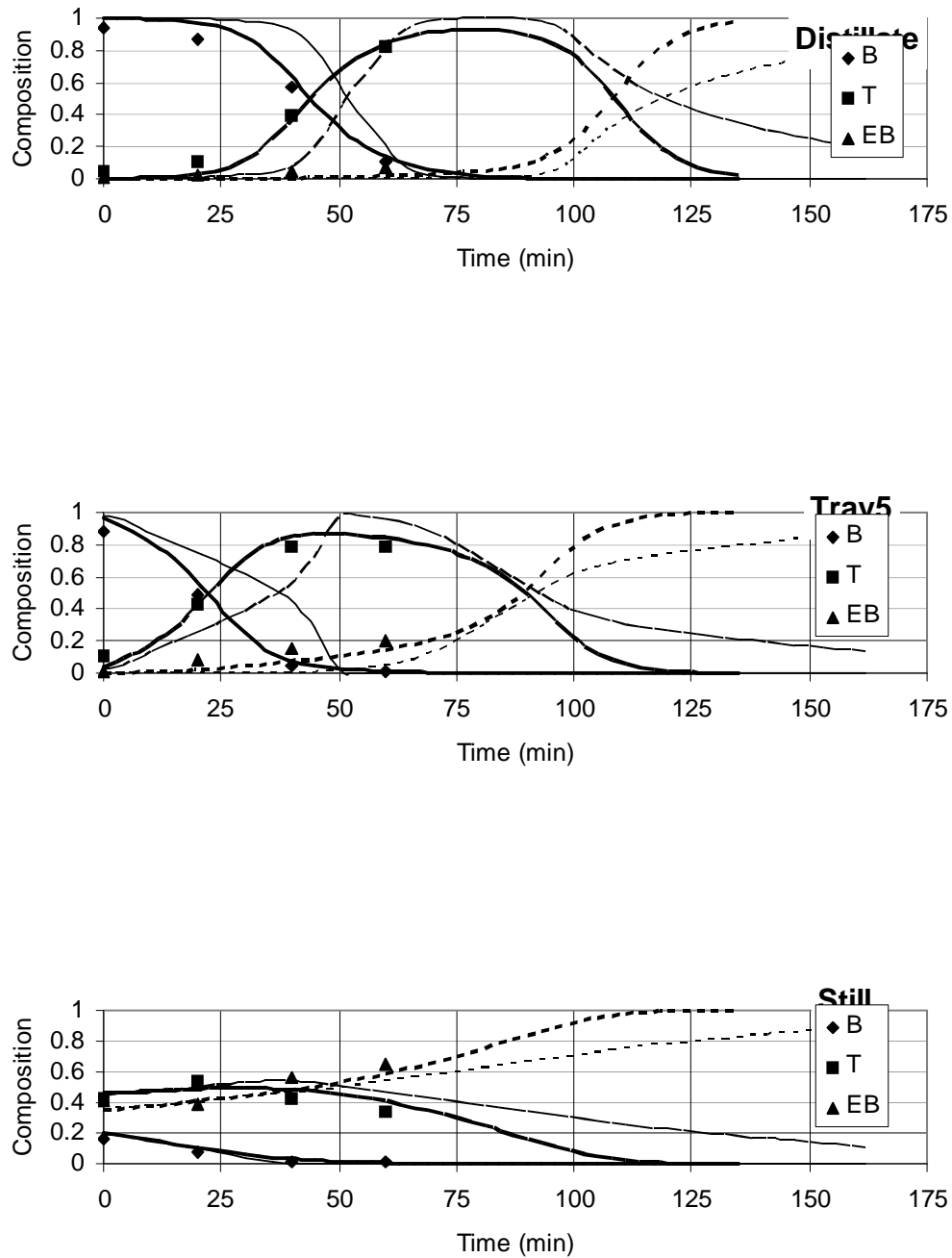
Figure (8): Experimental and Simulation Results of Equilibrium and Nonequilibrium Models Experiment no-3 Table (3). (Points \equiv Exp., Soft lines \equiv EQ model, and Bold Lines \equiv NEQ model)
