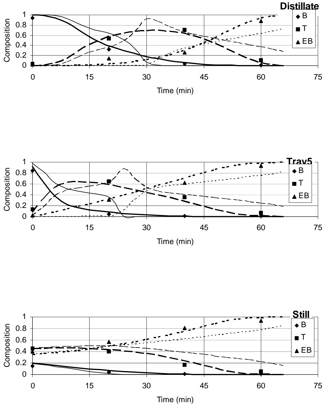
Figure (6): Experimental and Simulation Results of Equilibrium and Nonequilibrium Models Experiment no-1 Table (3).
