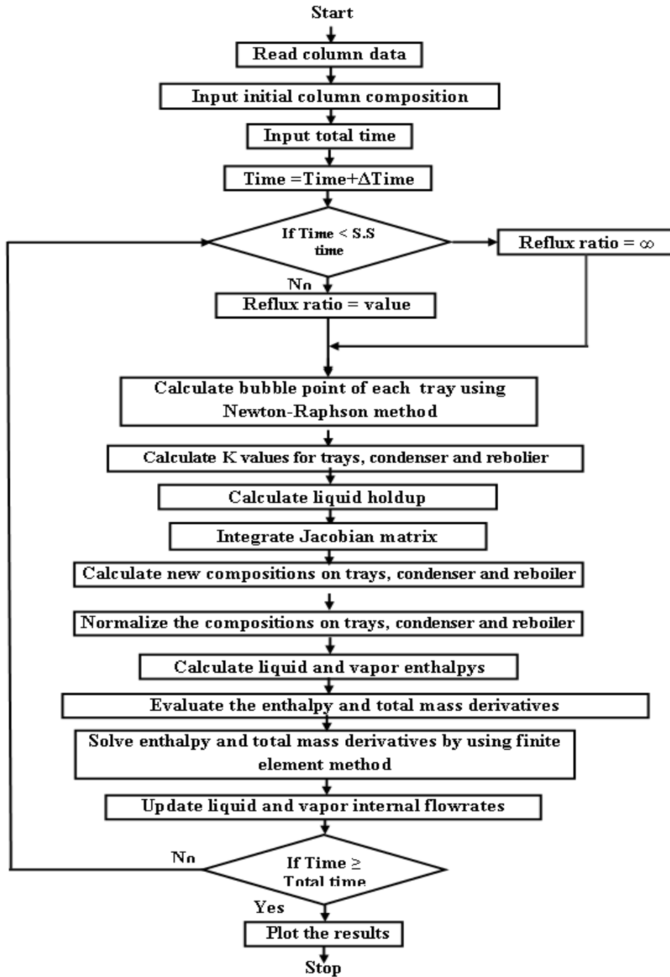
Figure (3): The Flow Chart of Solution Steps of equilibrium Stage Model
