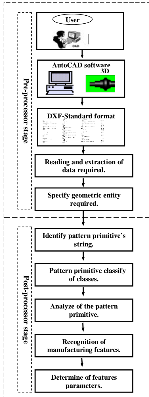
Figure (4) manufacturing features extraction and recognition algorithm.
