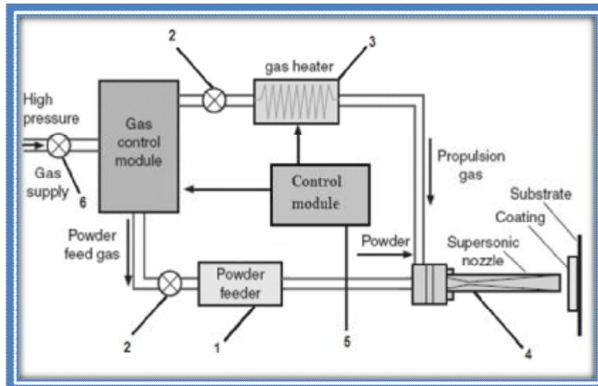
Figure.(1) Schematic diagram of cold spray system: 1. Powder feeder; 2.Two electric valves; 3. Heater. (To heat the carrier gas); 4. De Laval-type nozzle; 5. Control module; 6. Gas regulator.
