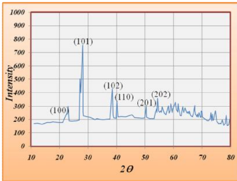
Figure.(3) The XRD patterns of the Te microtubes.
