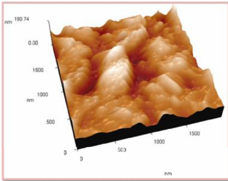
Figure.(5) AFM image of Te microtubes onto glass substrate at 200°C.
