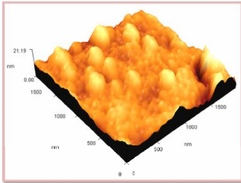
Figure.(6) AFM images of TeO 2 microtubes onto glass substrate at 200°C.
