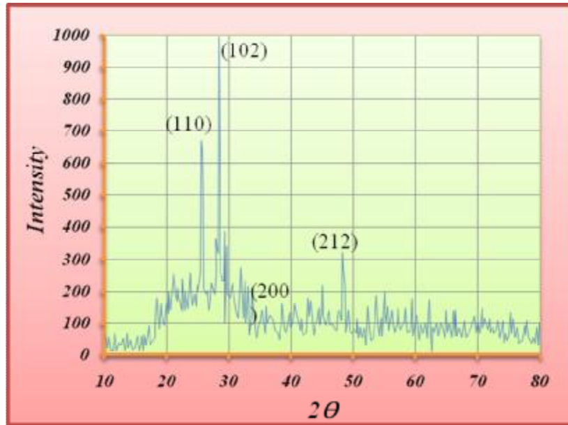
Figure.(4) The XRD patterns of the TeO 2 microwires.
