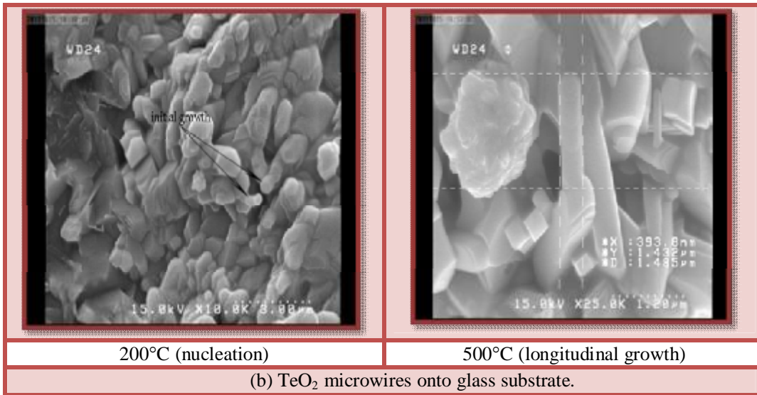
Figure.(7) SEM images of Te microtubes and TeO 2 microwires onto glass substrate.
