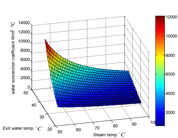
Figure(15) The effect of the exit cooling water and steam temperatures on convection heat transfer coefficient of water.
