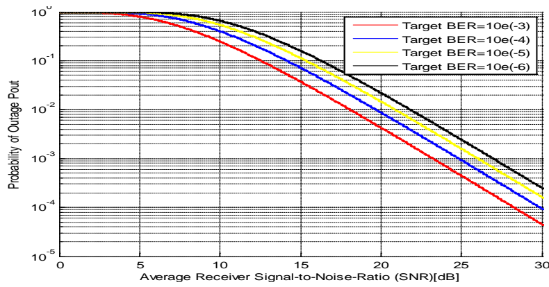
Figure (19) Outage probability for Nakagami fading (m=2)
