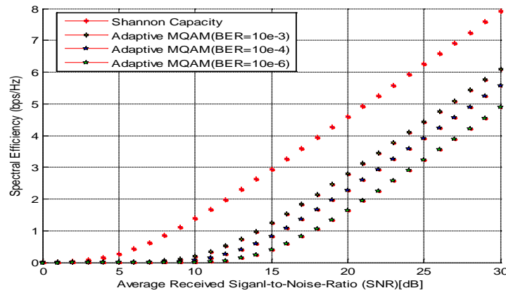
Figure (15) Spectral efficiency of Adaptive MQAM (Variable-rate Variable-power) in the presence of Nakagami fading ( m=2 ) for P_b = 10^{-3}, 10^{-4} & 10^{-6} .
