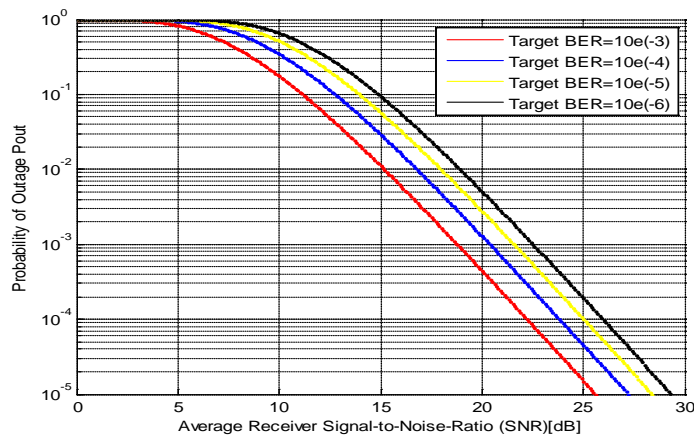
Figure (20) Outage probability for Nakagami fading (m=3)
