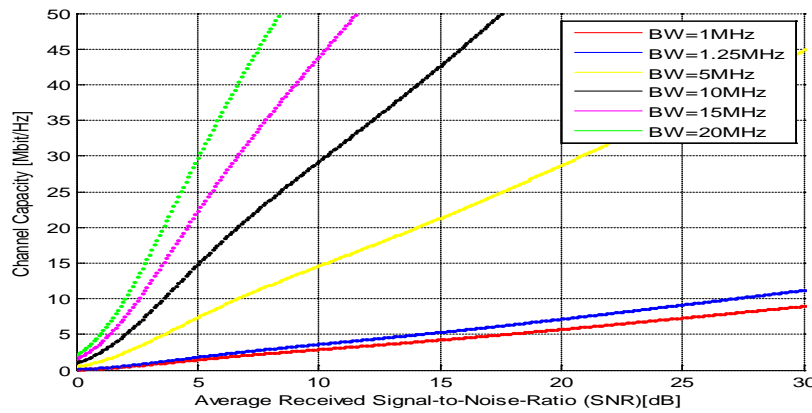
Figure (10) Channel capacity versus average received (S/N) for WiMax system with Truncated channel Inversion in the presence of Nakagami fading channel ( m=2 ).
