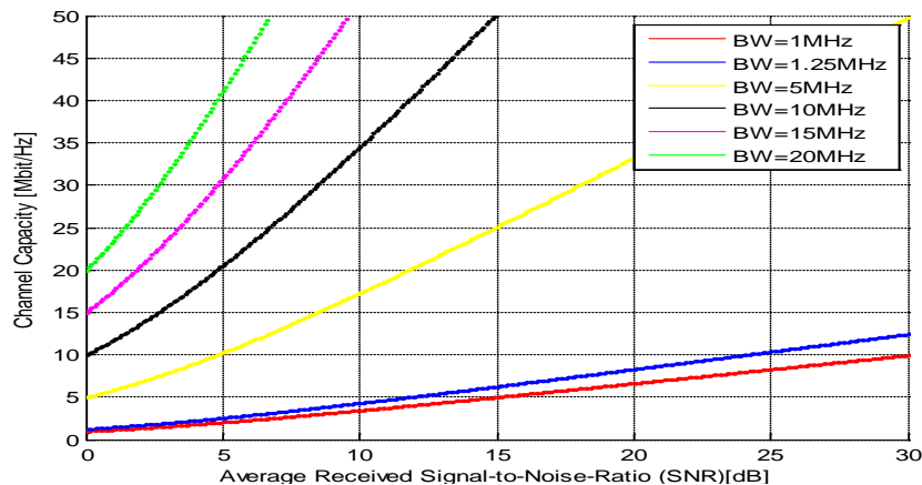
Figure (8) Channel capacity versus average received (S/N) for WiMax system with Variable- rate & Constant power in the presence of Nakagami fading (m=3).
