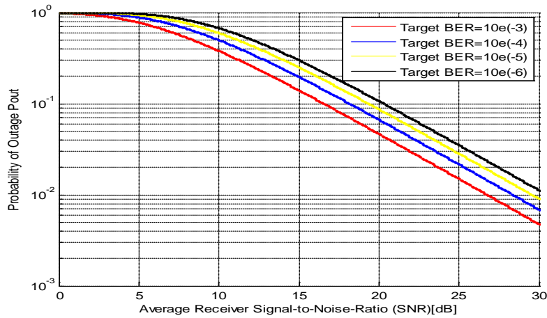
Figure (18) Outage probability for Rayleigh fading
