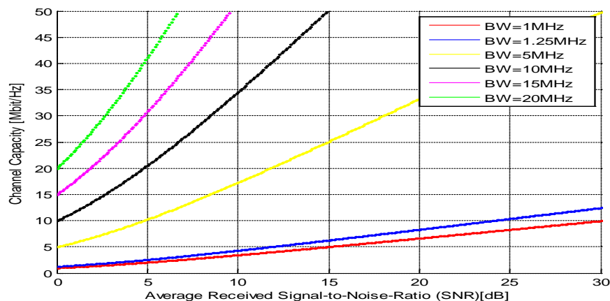
Figure (2) Channel capacity versus average received (S/N) of WiMax system in the presence AWGN.
