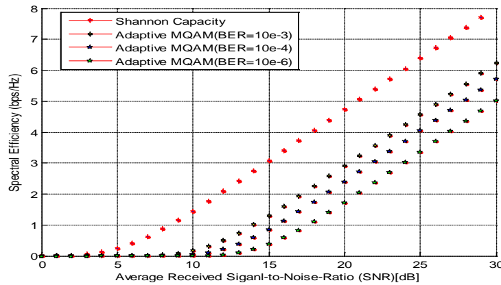
Figure (16) Spectral efficiency of Adaptive MQAM (Variable-rate Variable-power) in the presence of Nakagami fading ( m=3 ) for P_b = 10^{-3}, 10^{-4} & 10^{-6} .
