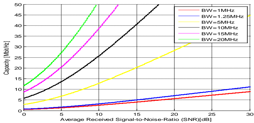
Figure (12) Channel capacity versus average received (S/N) for WiMax system with Total channel Inversion in the presence of Nakagami fading (m=2).
