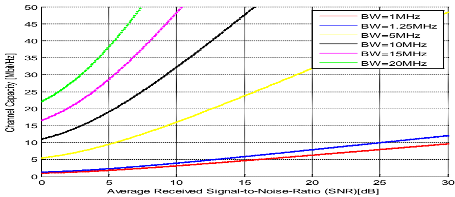
Figure (3) Channel capacity versus average received (S/N) for WiMax system with Variable- rate & Variable power in the presence of Rayleigh fading.
