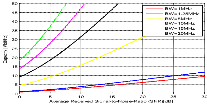
Figure (7) Channel capacity versus average received (S/N) for WiMax system with Variable- rate & Constant power in the presence of Nakagami fading (m=2).
