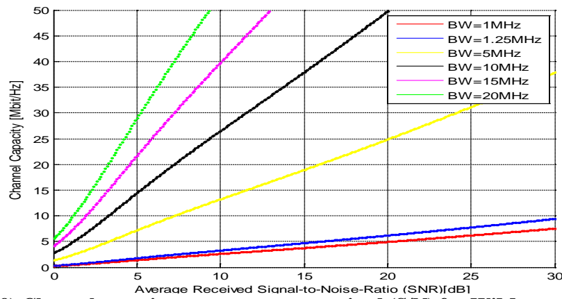
Figure (9) Channel capacity versus average received (S/N) for WiMax system with Truncated channel Inversion in the presence of Rayleigh fading ( m=1 ).
