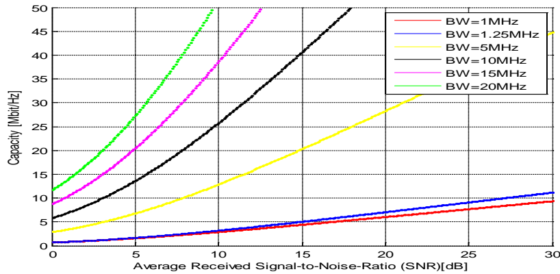
Figure (13) Channel capacity versus average received (S/N) for WiMax system with Total channel Inversion in the presence of Nakagami fading (m=3).
