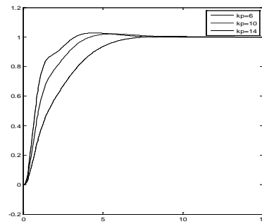
Figure.(8) step responses of P4 for three values of k_p .
