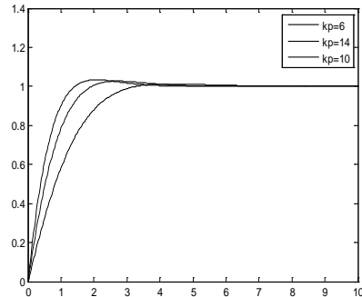
Figure.(6) step responses of P2 for three values of k_p .
