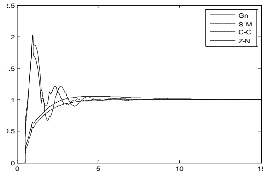
Figure (4) step responses for P1 for the four controllers of comparison study.
