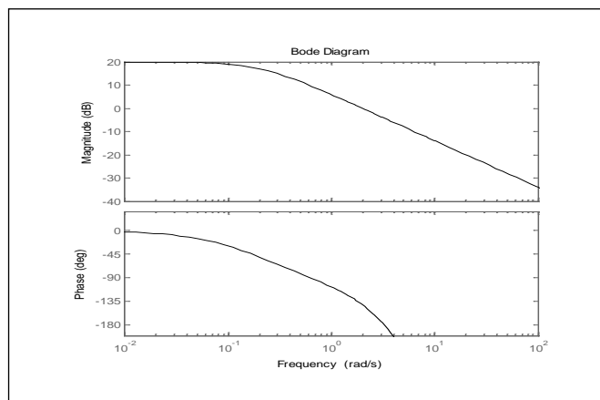
Figure (3) Bode plot for the model p1.
