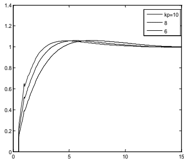
Figure.(5) step responses for P1 for three values of k_p .
