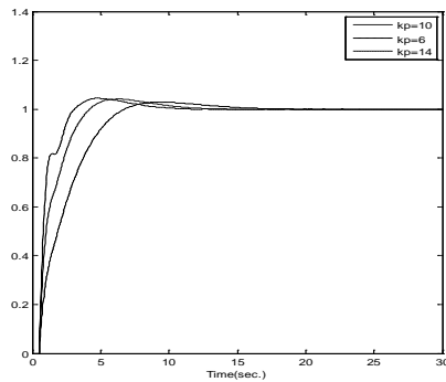
Figure.(7) step responses of P3 for three values of k_p .
