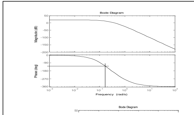
Figure (2) Bode plot for a certain plant model .
