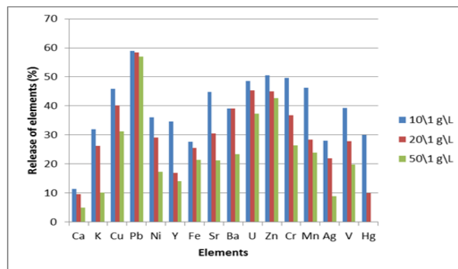
Figure 4: Effect of Solid to Liquid ratio on removed heavy and radioactive elements from Phosphogypsum by deionized water
