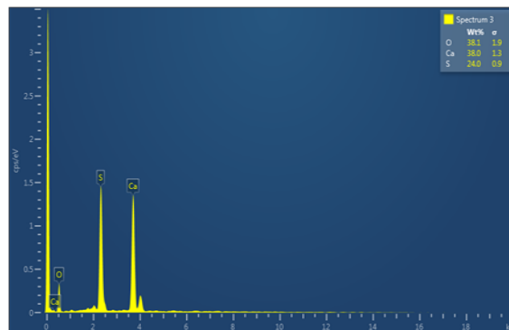
Figure 2: SEM inspection of the phosphogypsum ore
