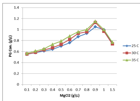
Figure 7: Solubility of phosphogypsum in aqueous solutions of MgCl_2 .
