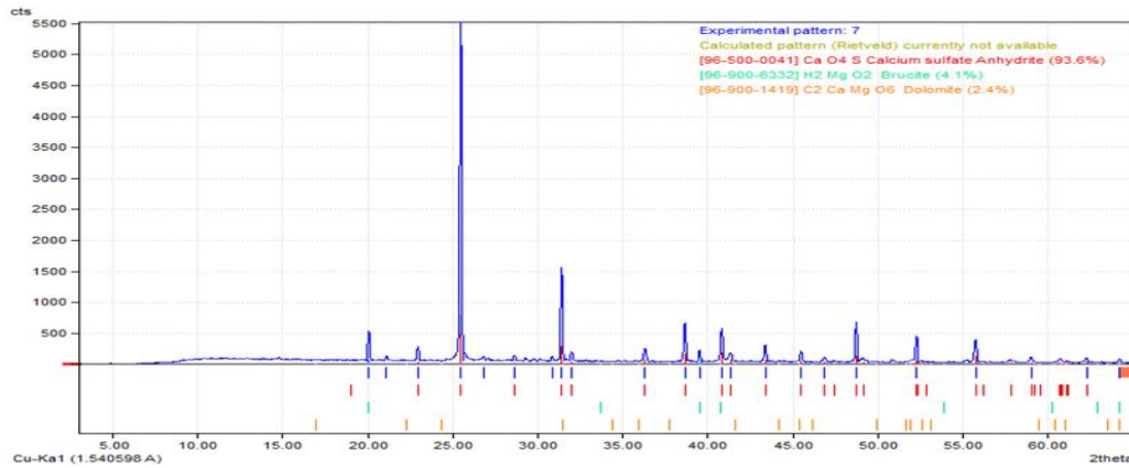
Figure 1: XRD pattern of the phosphogypsum
