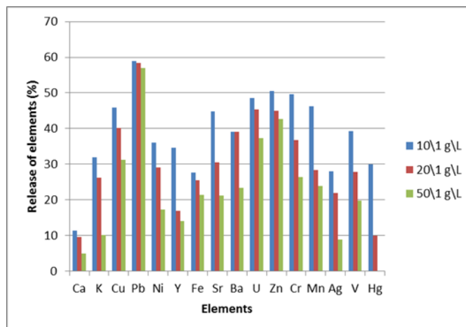
Figure 5: Effect of Temperatures on removed heavy and radioactive elements from Phosphogypsum by deionized water.
