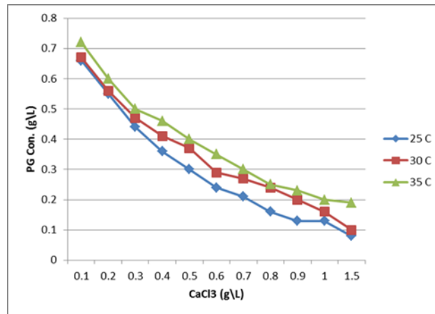
Figure 8: Solubility of phosphogypsum in aqueous solutions of \text{CaCl}_2 .
