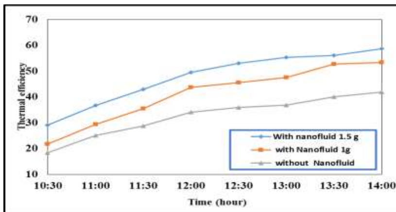
Figure 7: Thermal efficiency at different concentration
