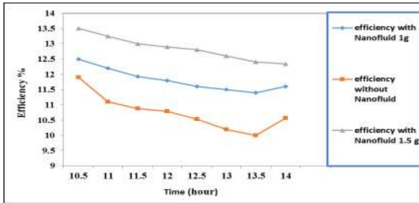
Figure 6: Efficiency of PV with time
