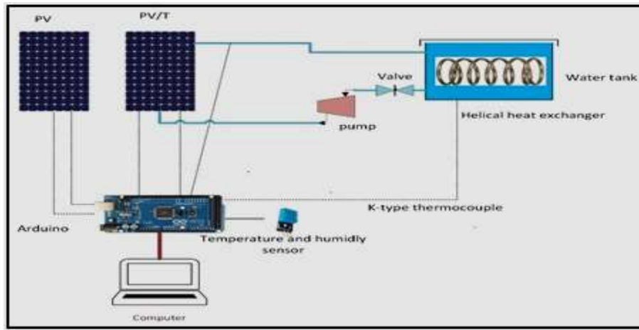
Figure 2: Schematic diagram of proposed PVT arrangement
