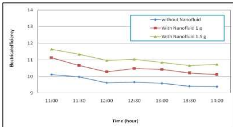
Figure 8: Electrical efficiency at different concentration
