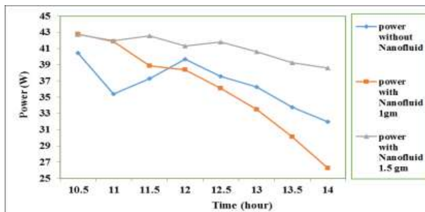
Figure 9: Power at different concentration
