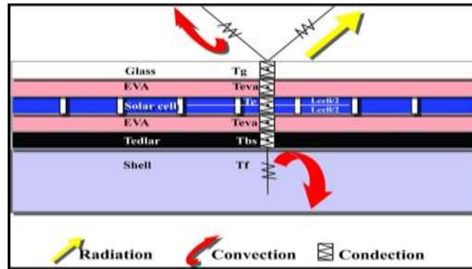
Figure 1: Heat transfer modes and equivalent thermal network
