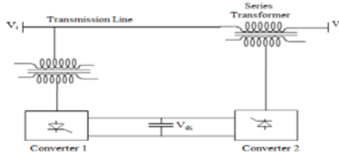
Figure 1: The UPFC structure [3]
