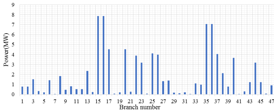
Figure 7: Active power losses without UPFC
