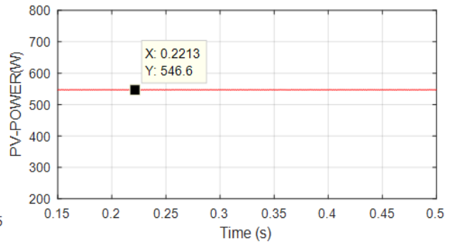
Figure 8: P_{pv} @ 400W/m^2, 60^\circ C R_L(100\Omega)
