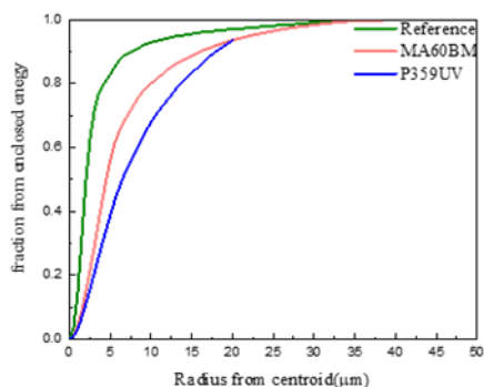
Figure 5: The encircled energy collected by the IOLs compared with the reference LBEM
