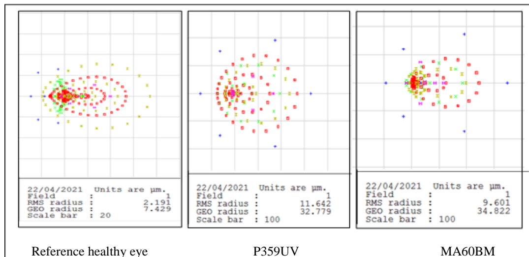
Figure 4: Polychromatic spot diagram for models' eye with refractive IOLs implanted
