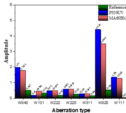
Figure 6: monochromatic aberration of (LBEM) and refractive IOL
