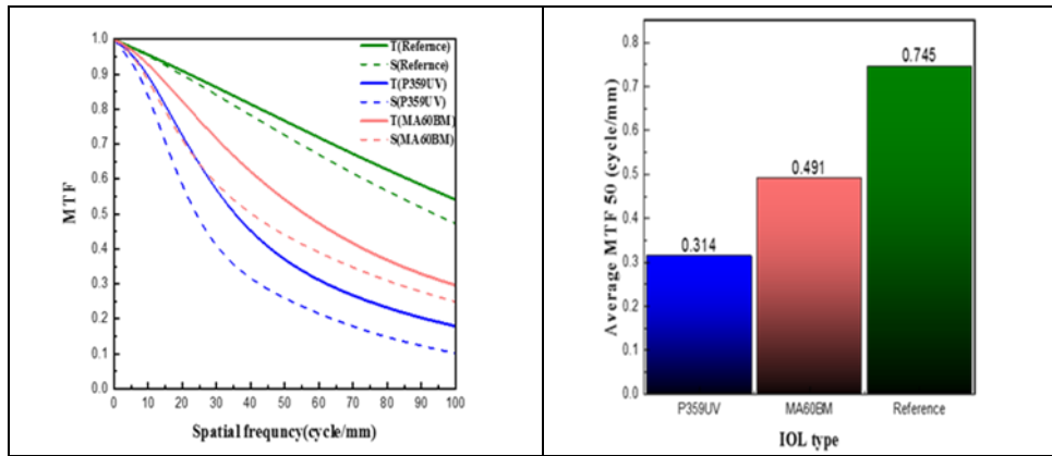
Figure 3: The modulation transfer function comparison between refractive lenses and (LBEM) model, The Average MTF at the spatial frequency (50 cycle/mm)
