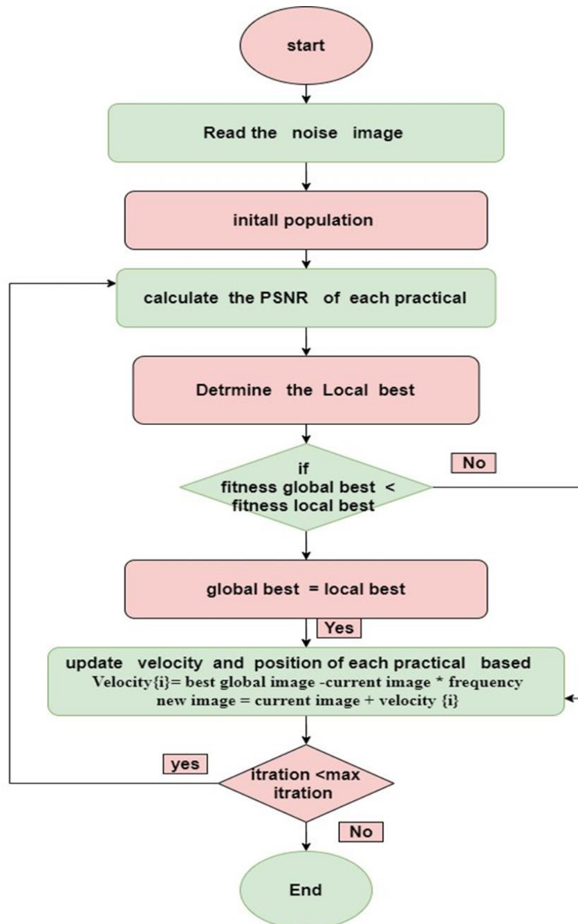
Figure 1: The flowchart of Denise of the proposed method (Bat Algorithm)
