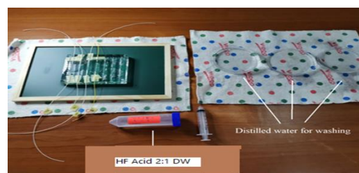
Figure 3: Chemical Etching
