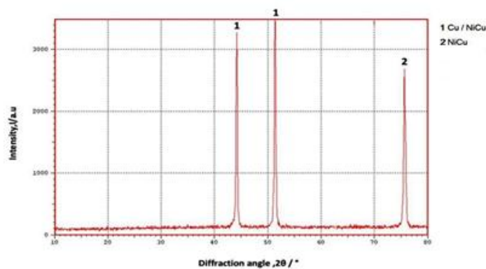
Figure 6: X-ray diffraction for the coating layer
