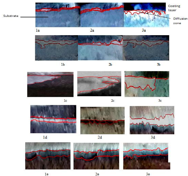
Figure 5: Optical microscope diffusion images 10X magnification power
