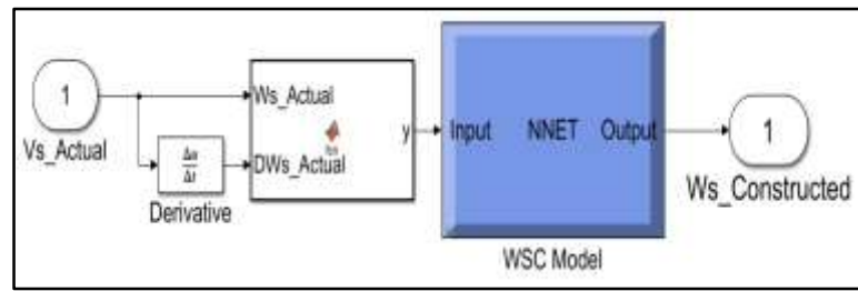
Figure 6: WSC Data Constructor model
