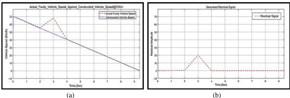
Figure 15: Injected Fault Test Results: (a) Faulty vs. Constructed Signals and (b) Generated residual signal
