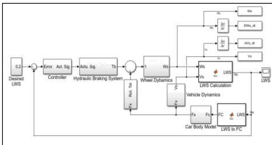
Figure 4: ABS Model Block Diagram
