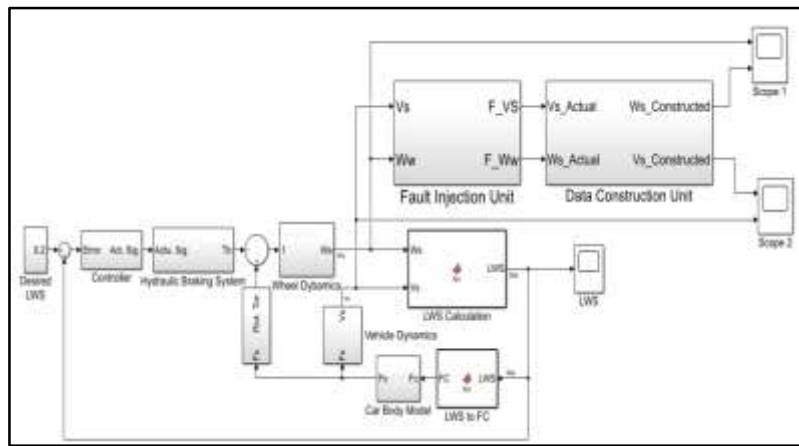
Figure 14: ABS model with Data Construction Unit and Fault Injection Unit
