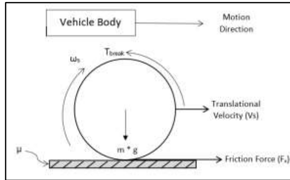
Figure 1: QCM model
