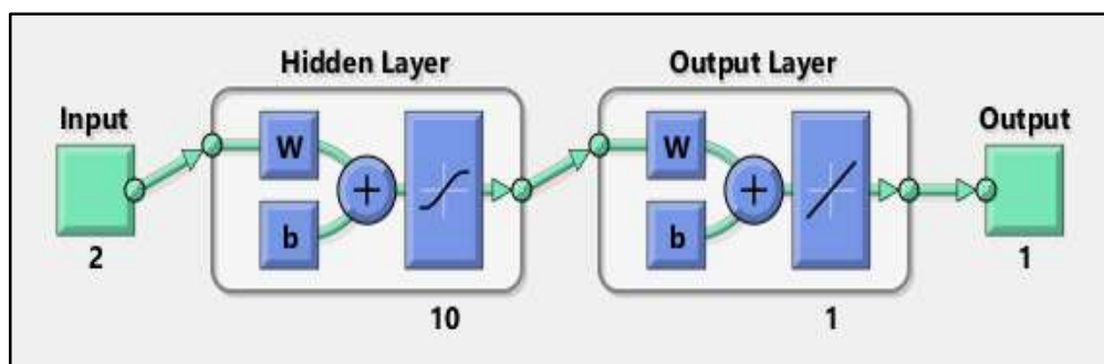
Figure 5: NN-MLP Based WSC Model Topology
