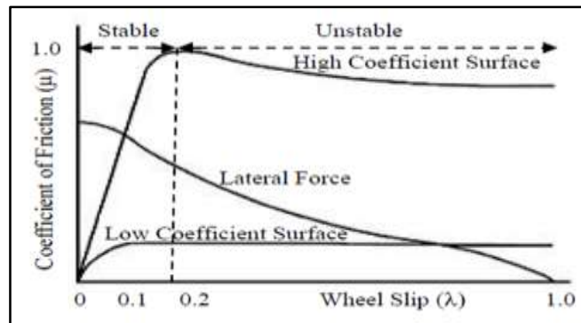
Figure 2: RFC ( \mu ) versus LWS ( \lambda )[21]
